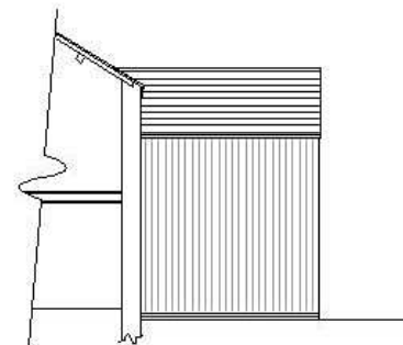
Part Elevation
