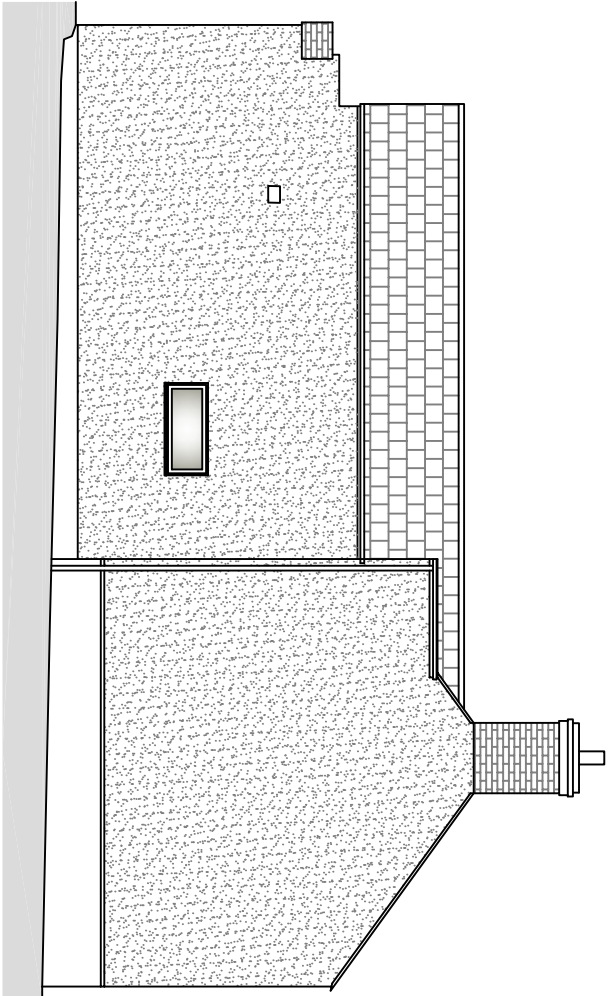
West Elevation 0 1 2 3m scale bar
