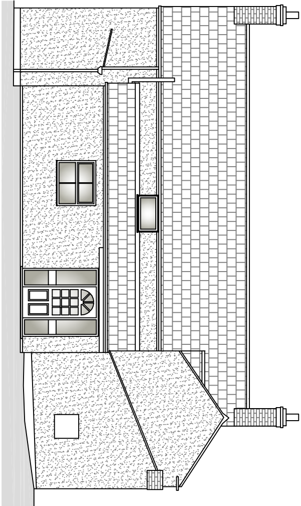
North Elevation 0 1 2 3m scale bar
