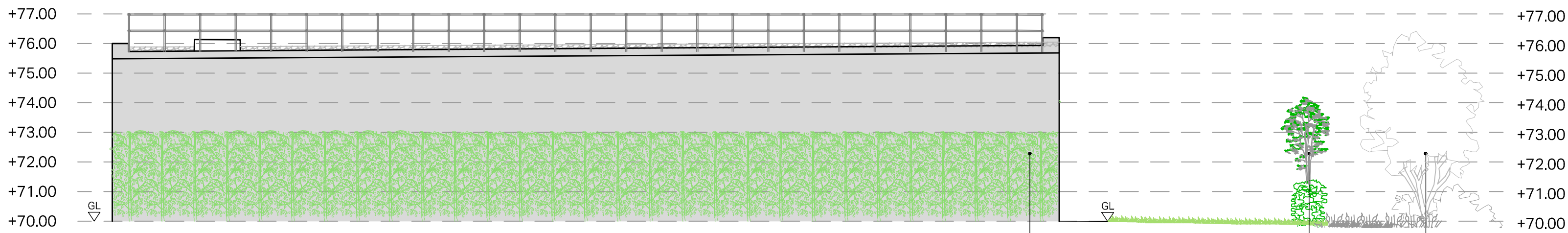
01 STAGE 1 RESERVOIR - ELEVATION FROM SOUTH - YEAR 0 SCALE: 1:125 @A1
