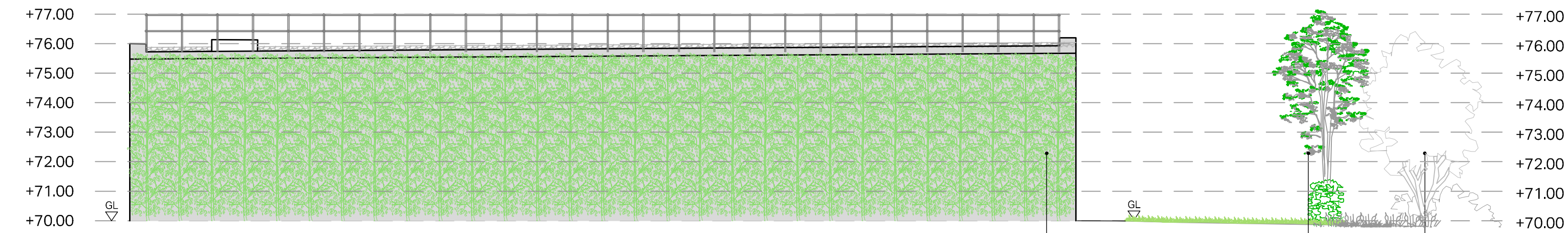
01 STAGE 1 RESERVOIR - ELEVATION FROM SOUTH - YEAR 8-10 APPROX SCALE: 1:125 @A1
