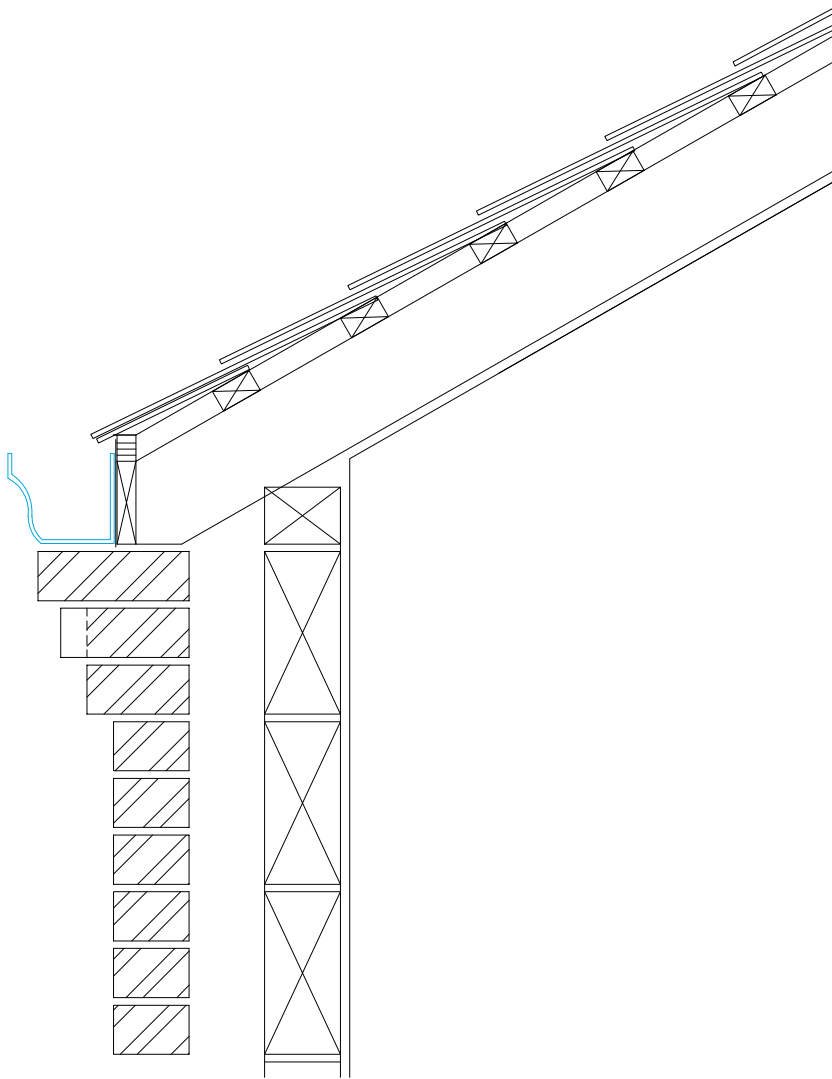
TYPICAL EAVES DETAIL ANCILLARY BUILDINGS
