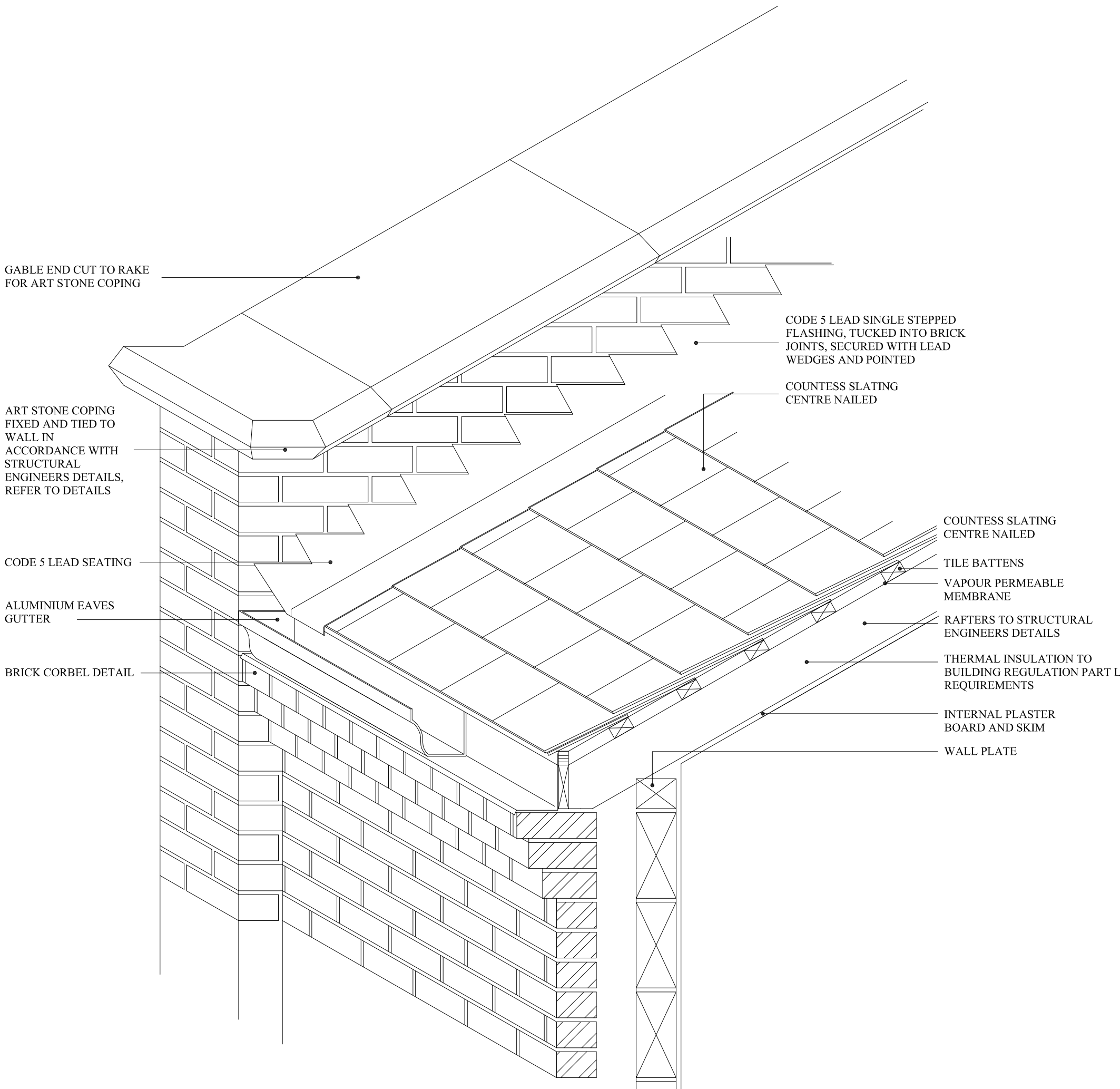
TYPICAL EAVES DETAIL ANCILLARY BUILDINGS
