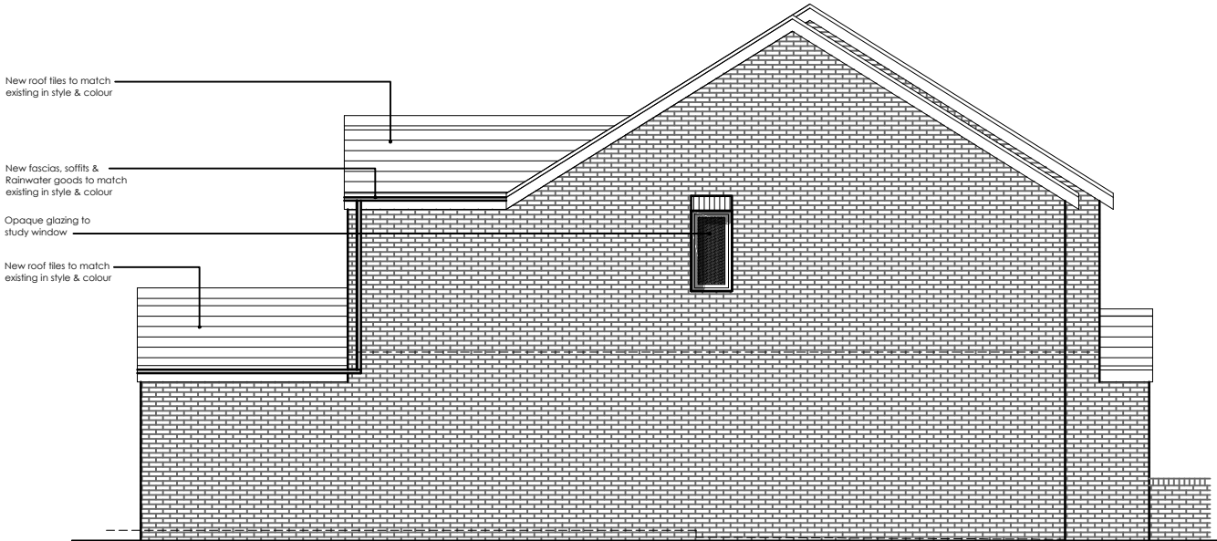
SIDE ELEVATION - 1:100
