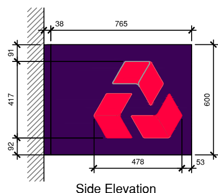
Projecting Sign
