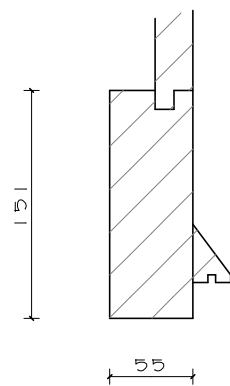
Vertical Section Scale 1 : 5
