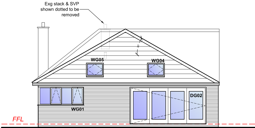
REAR ELEVATION
