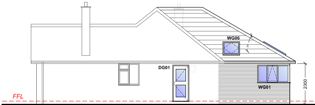
SIDE ELEVATION
