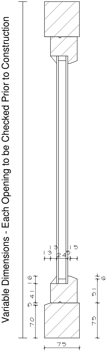
Vertical Section Detail 1 : 5
