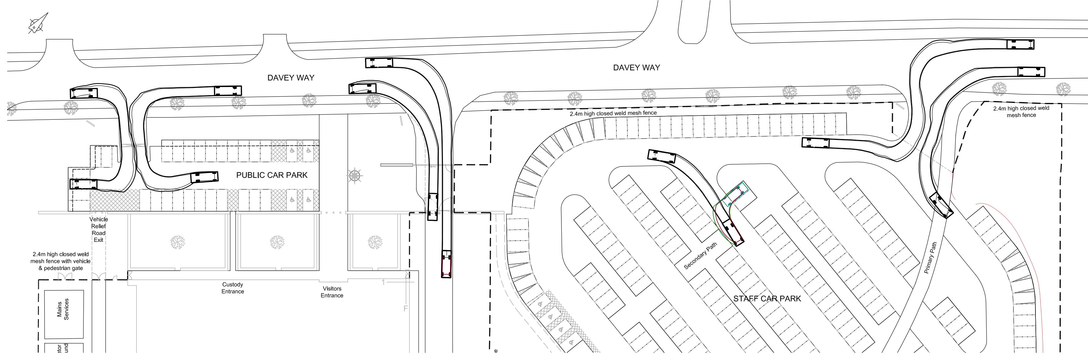
CAR PARKS, ENTRANCES & EXITS - LIGHT VAN SCALE : 1:500
