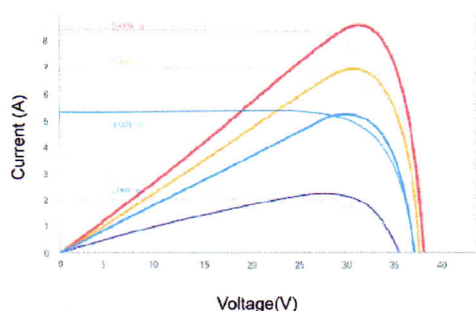
I-V Curves at different Irradiances
