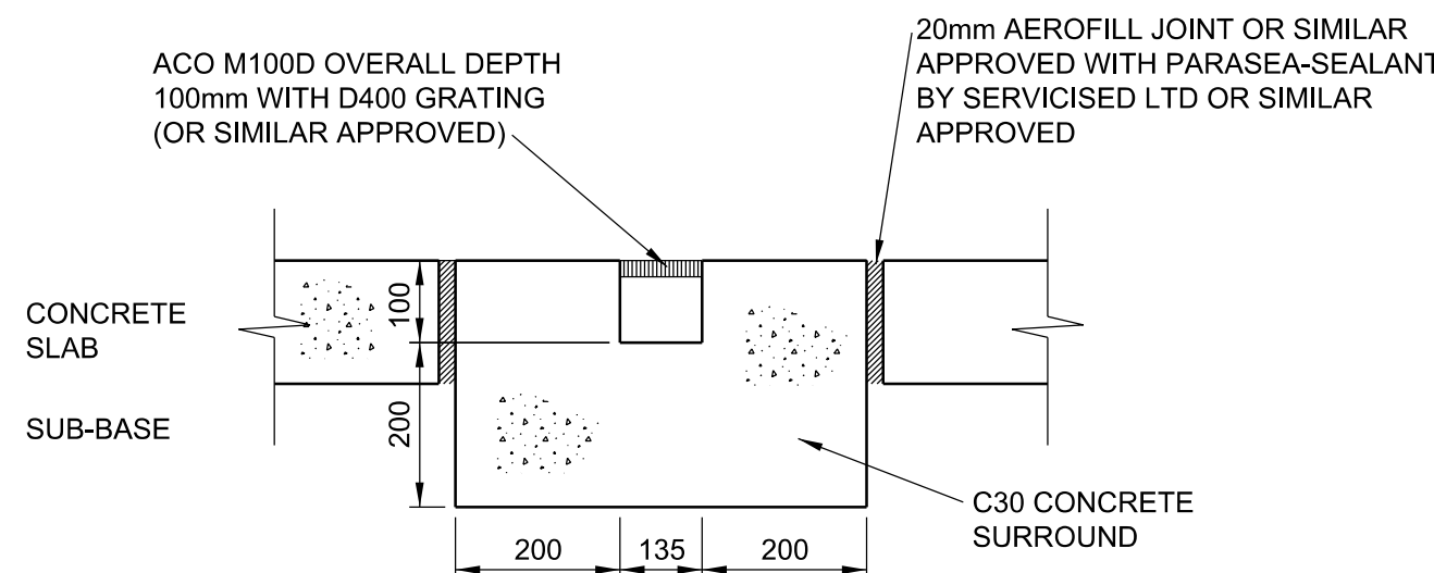
ACO CHANNEL DETAIL
