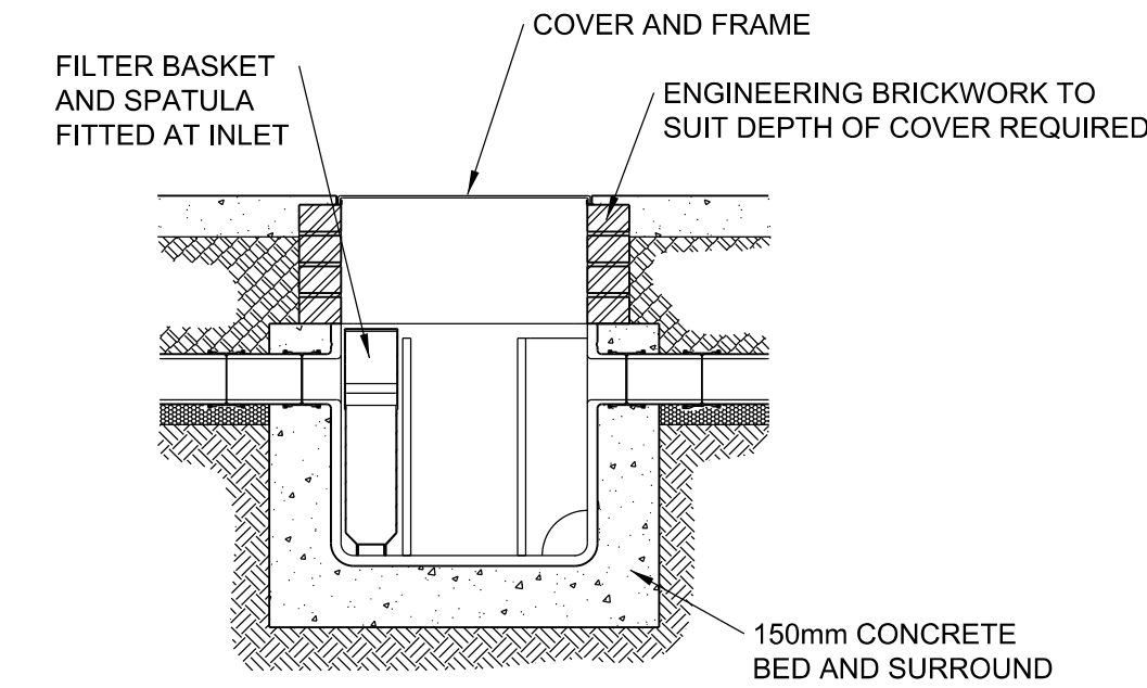
GREASE TRAP INSTALLATION DETAIL
