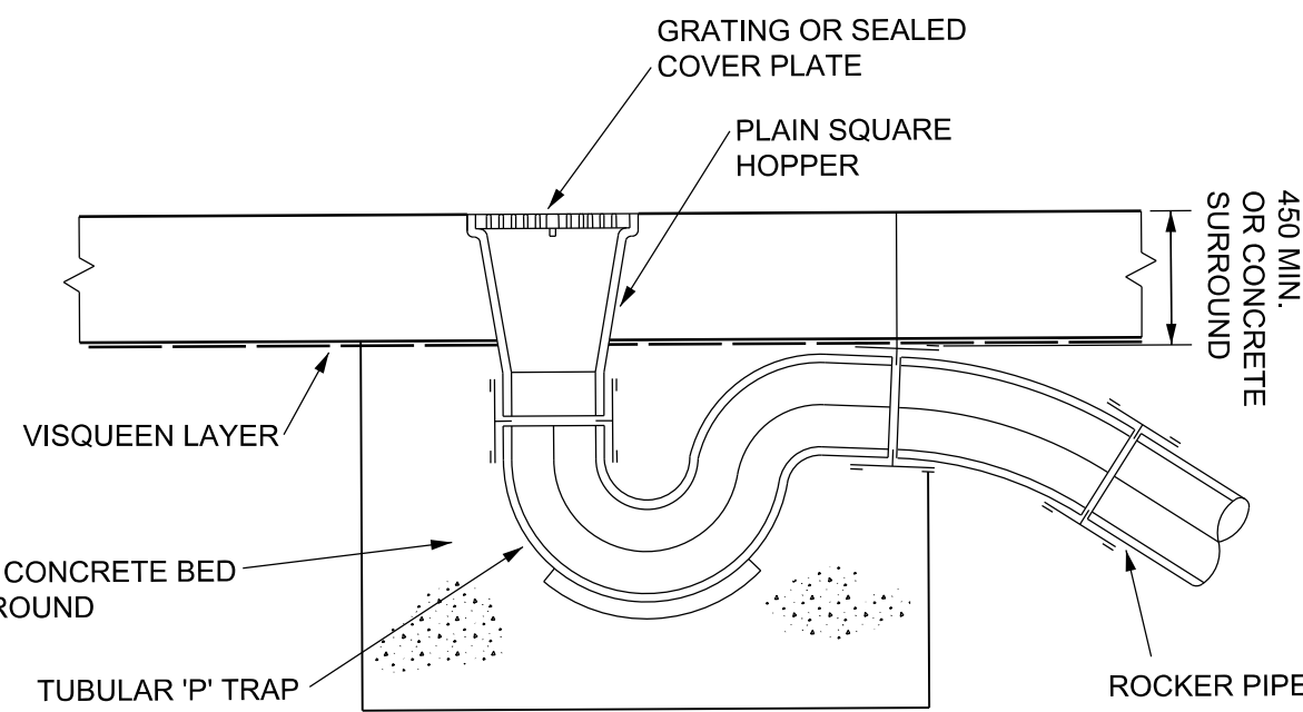
FLOOR GULLY
