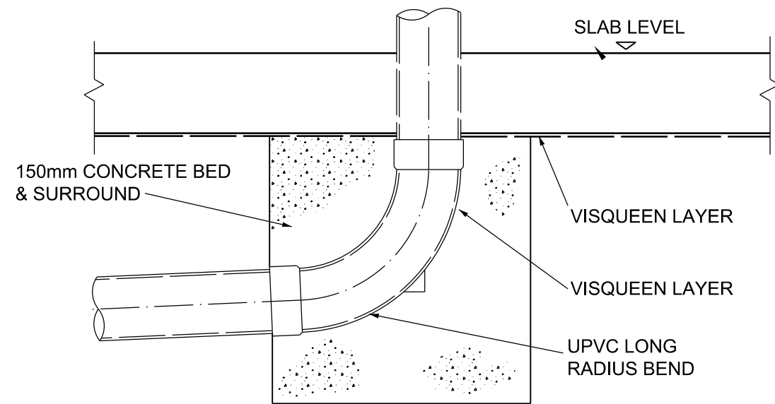
DRAINAGE CONNECTION DETAIL
