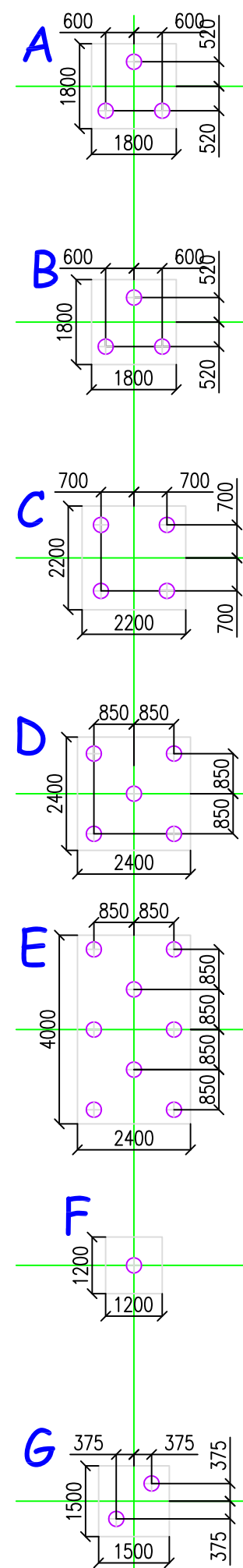
TYPICAL PAD FOUNDATION SETTING OUT DETAILS
