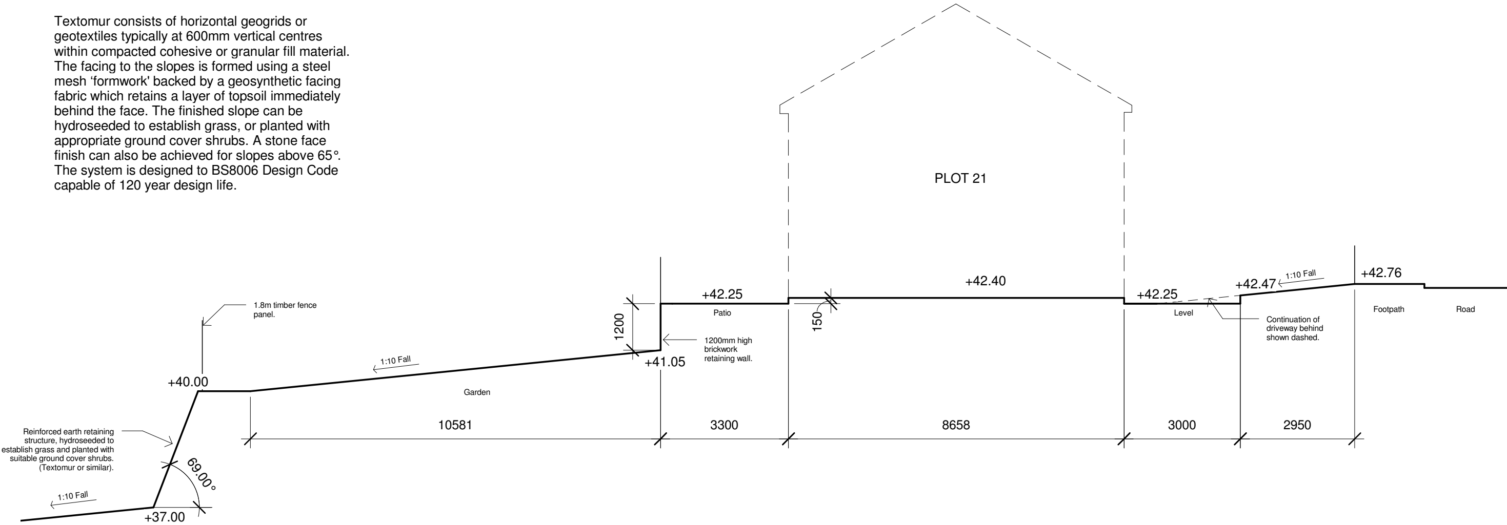
Typical Plot Section 1 : 100
