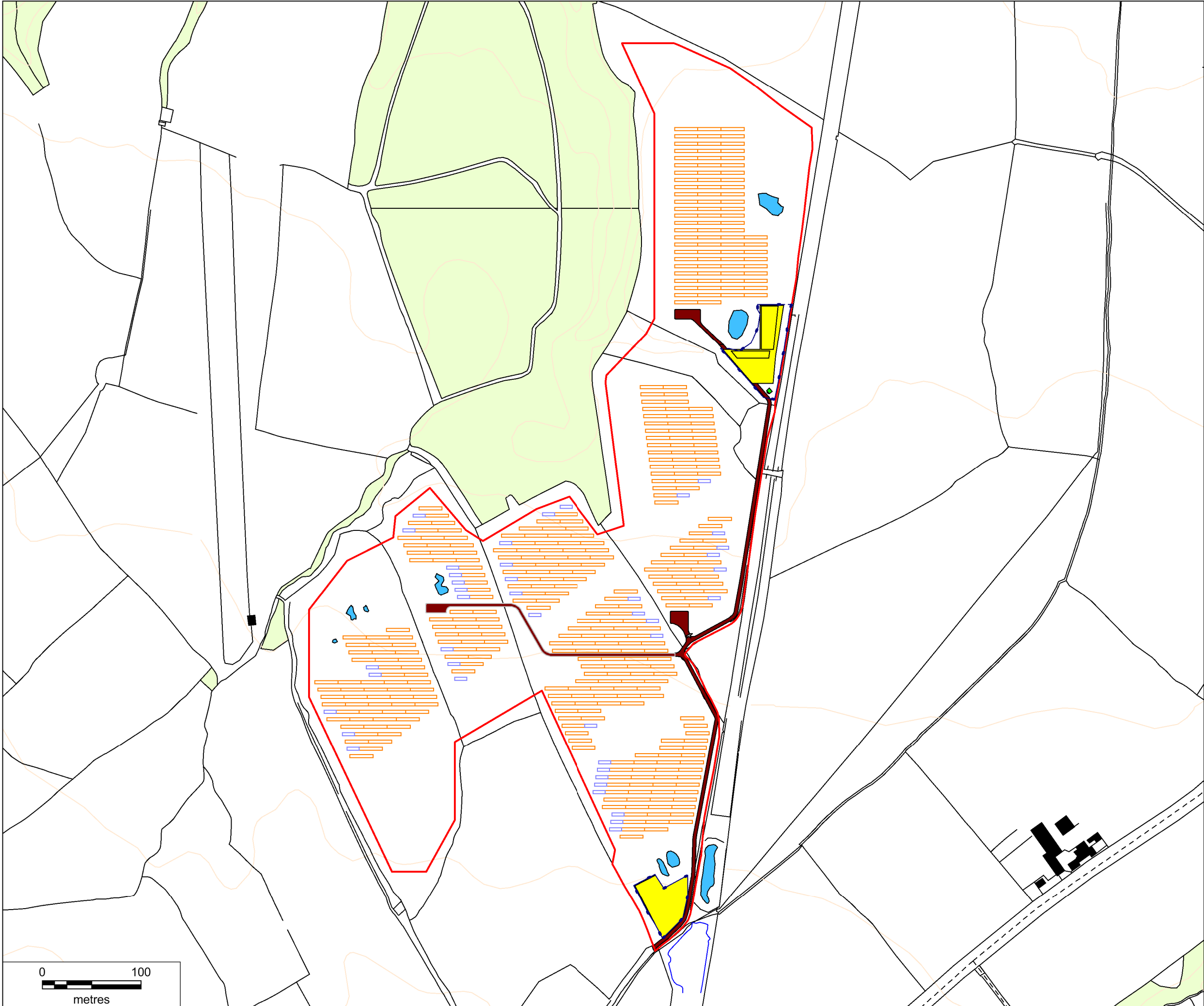
Figure 1 - Indicative Great Crested Newt Fencing Layout
