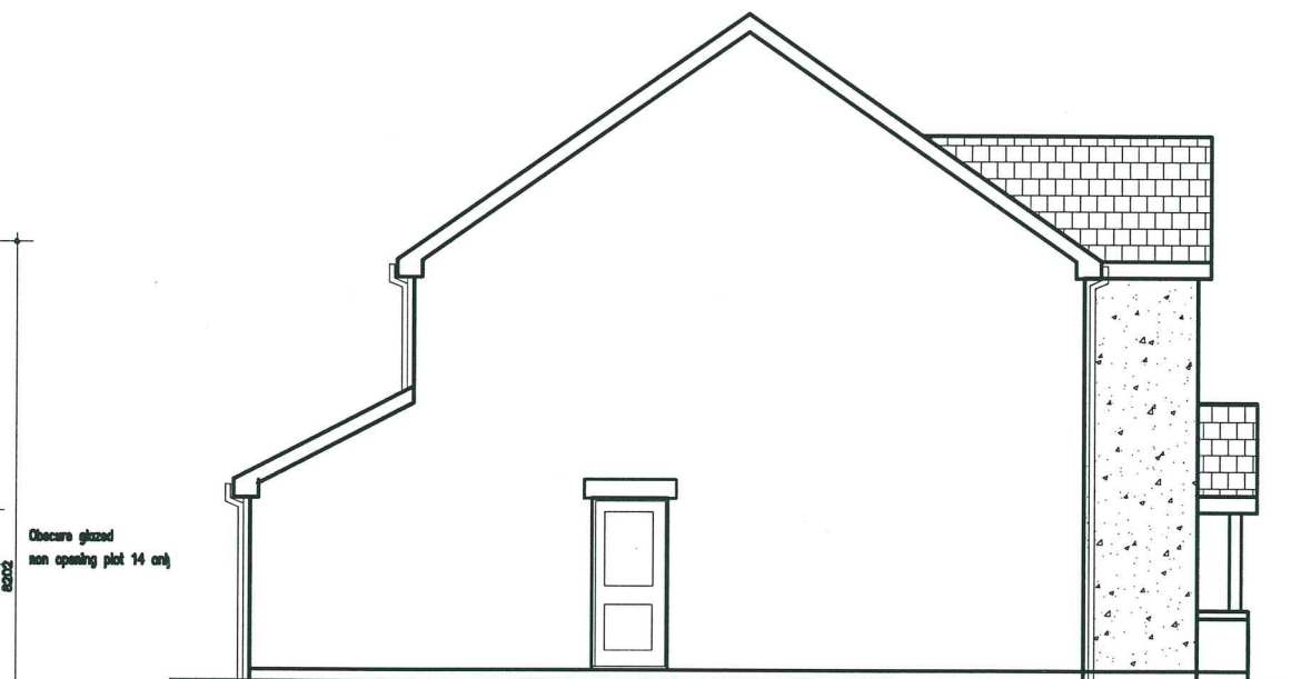
Side Elevation
