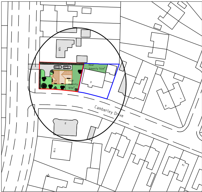
Location Plan 1:1250
