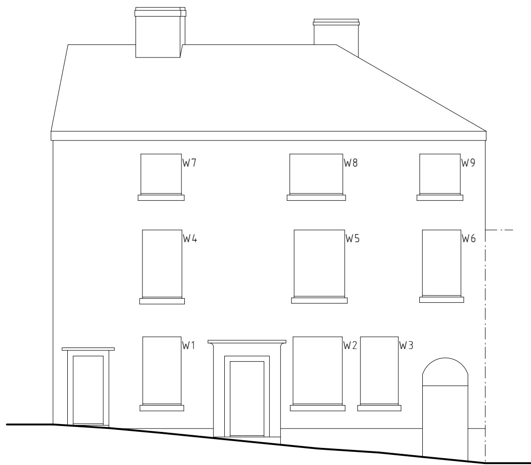
Front Elevation
