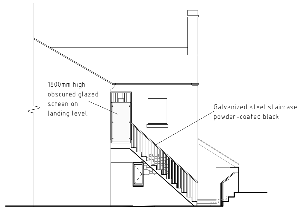
Part Side Elevation
