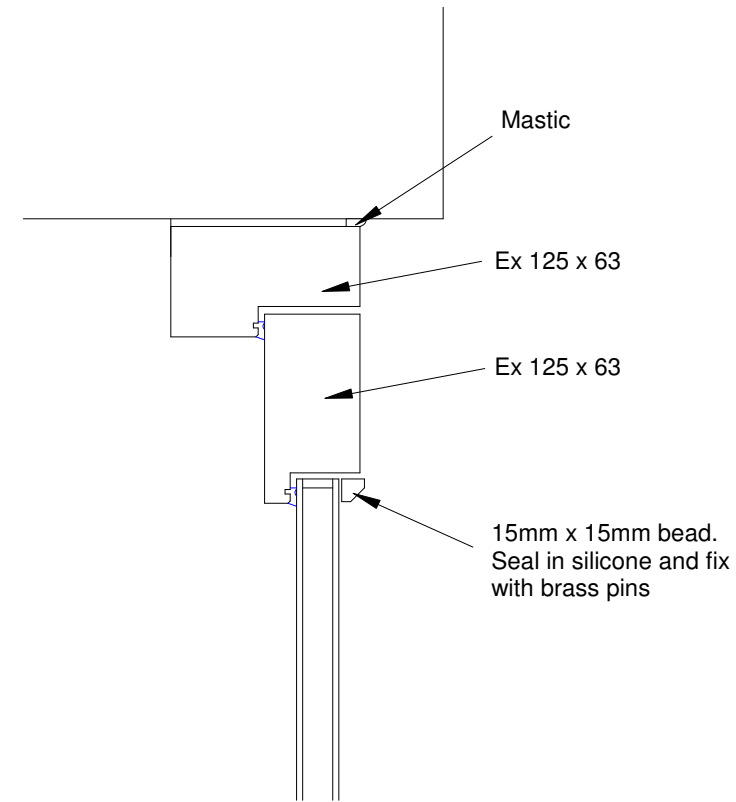
Detail D - 1:5
