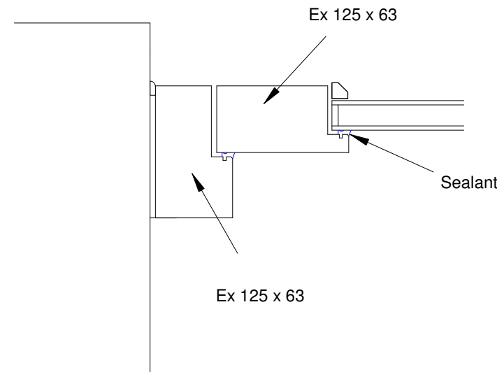
Detail C - 1:5
