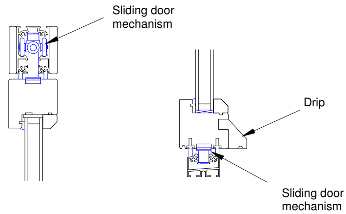
Detail A - 1:5
