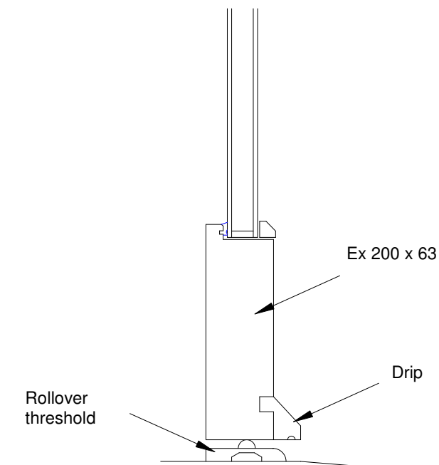
Detail E - 1:5
