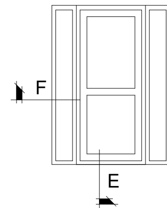
Window 3 1:50
