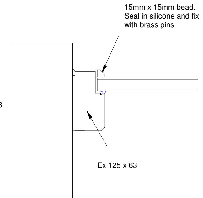
Detail F - 1:5
