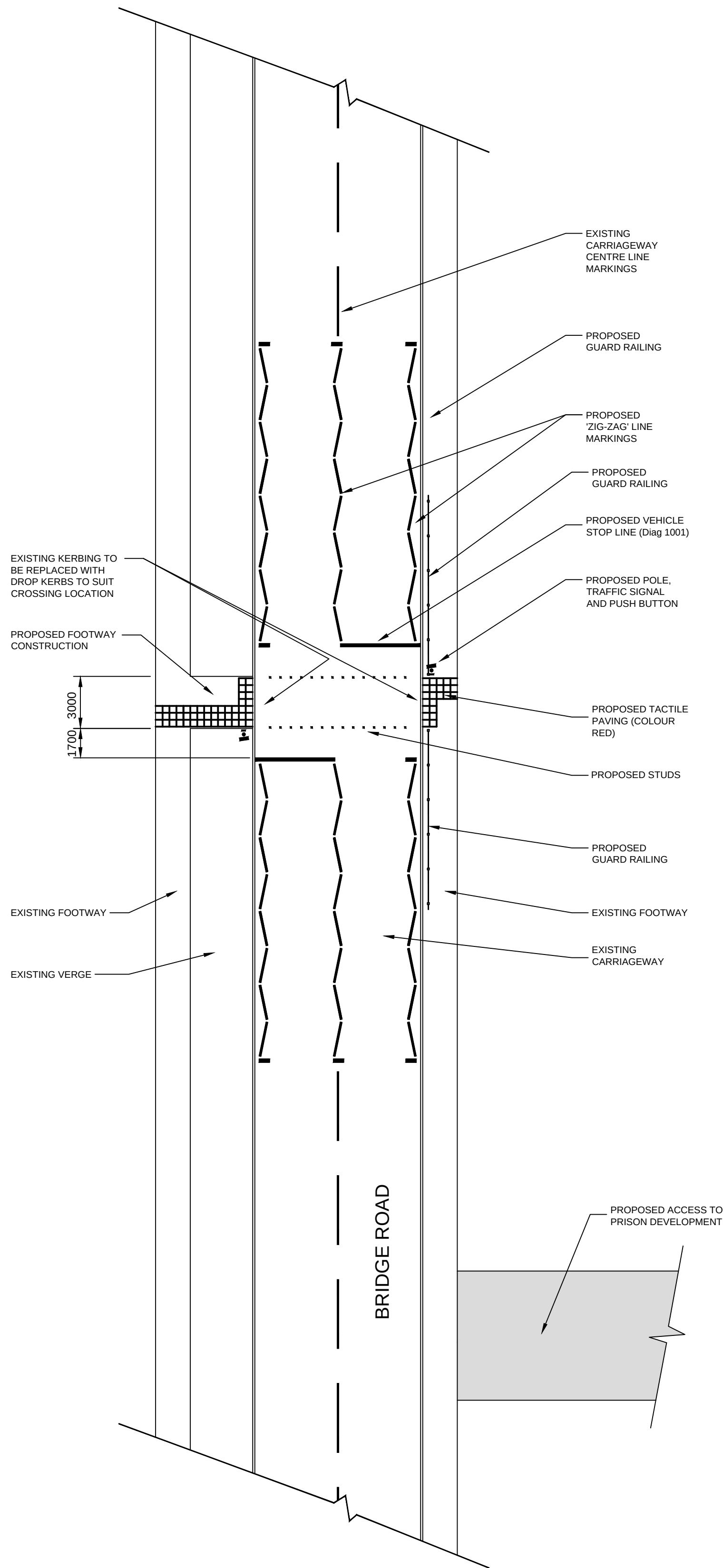
PEDESTRIAN (PUFFIN) CROSSING GENERAL ARRANGEMENT SCALE 1:200
