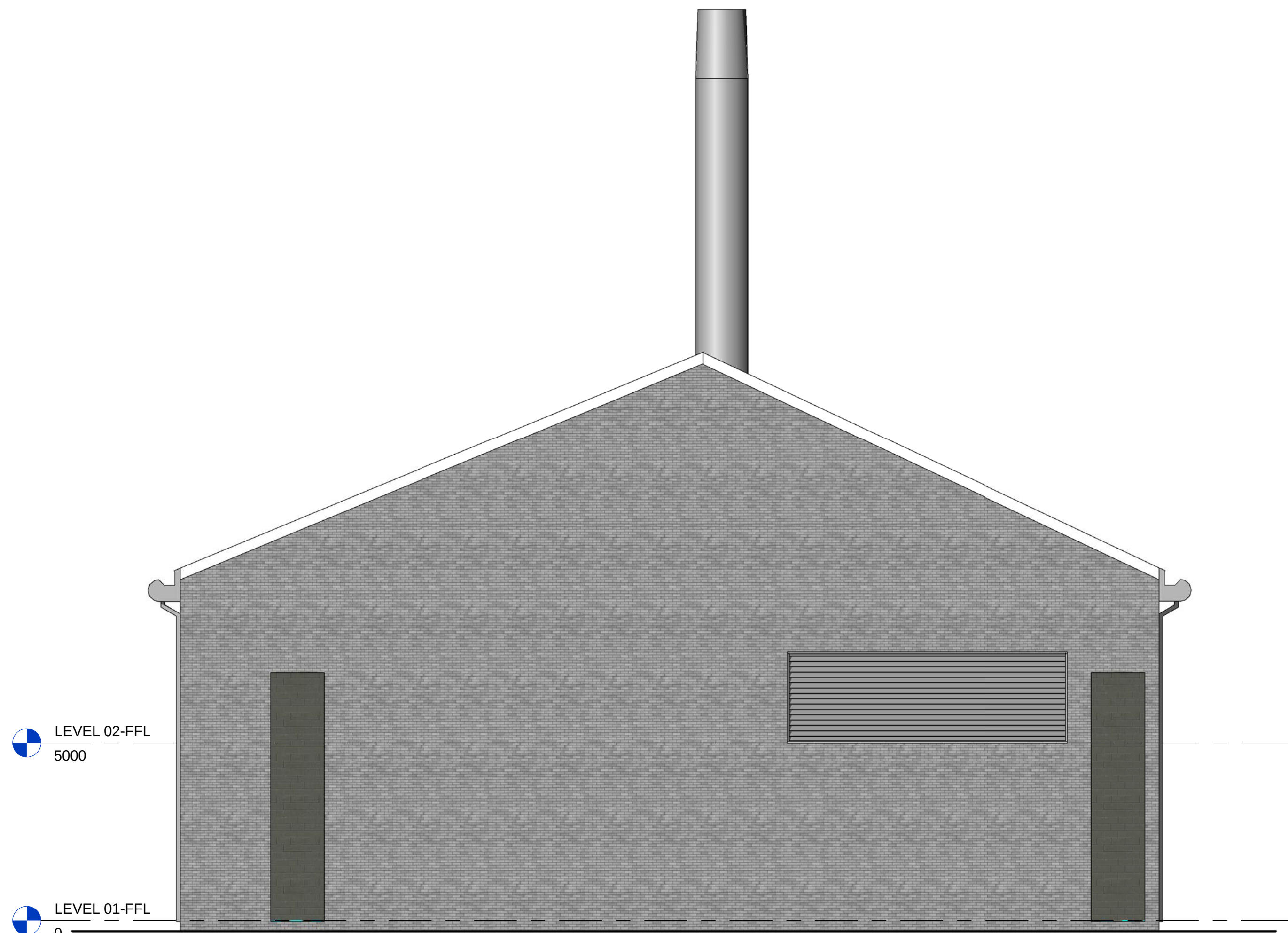
2 Elevation B (View from Vehicle Entry Lock) 1 : 100
