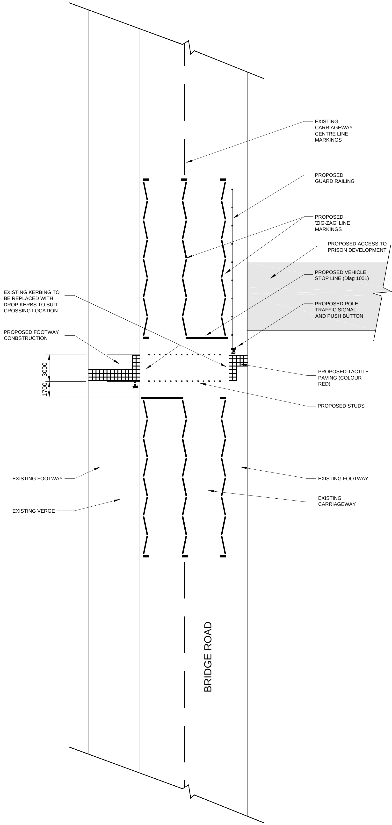
PEDESTRIAN AND CYCLIST CROSSING GENERAL ARRANGEMENT SCALE 1:200
