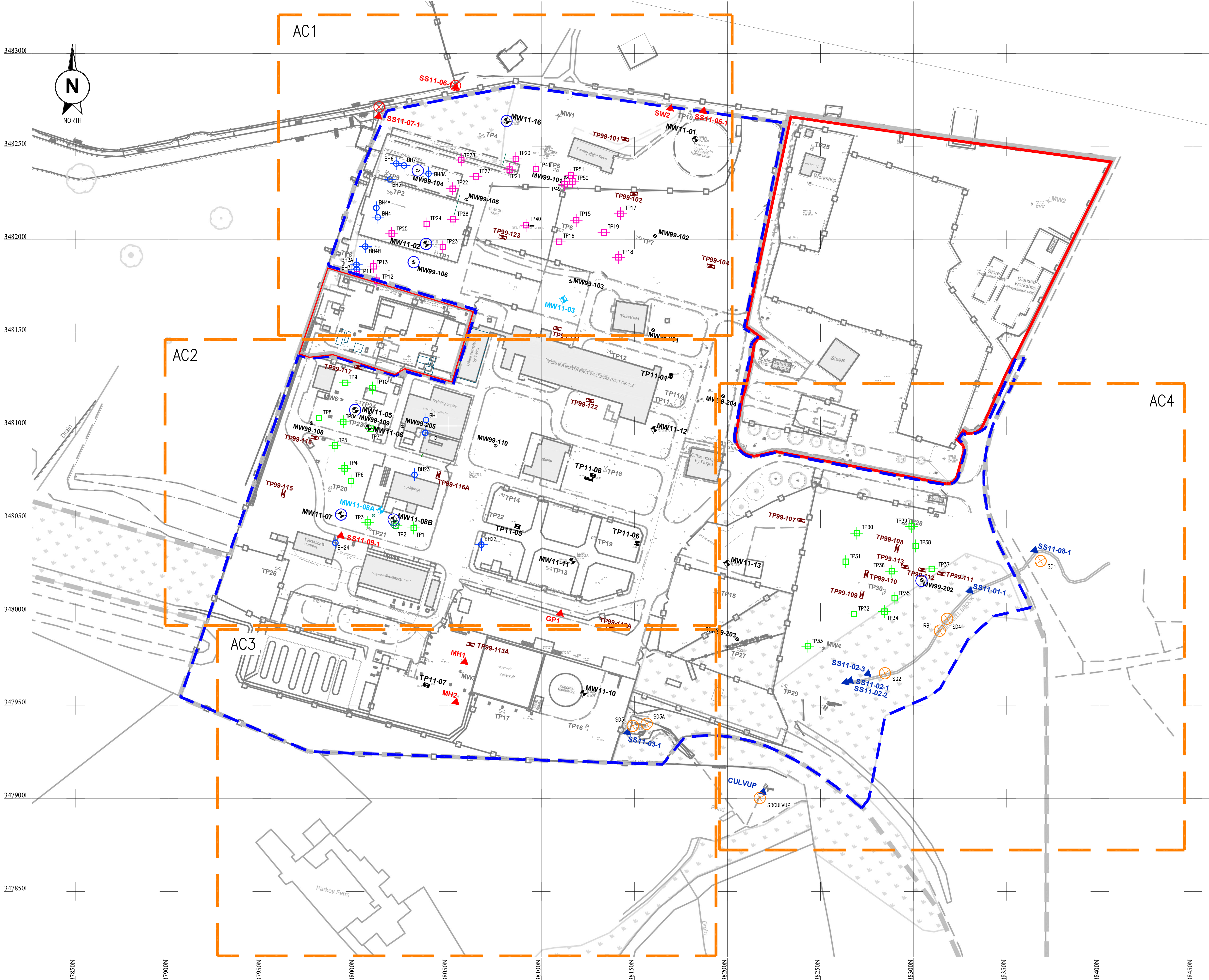
TILE LAYOUT PLAN - AREA AC SCALE 1:1000
