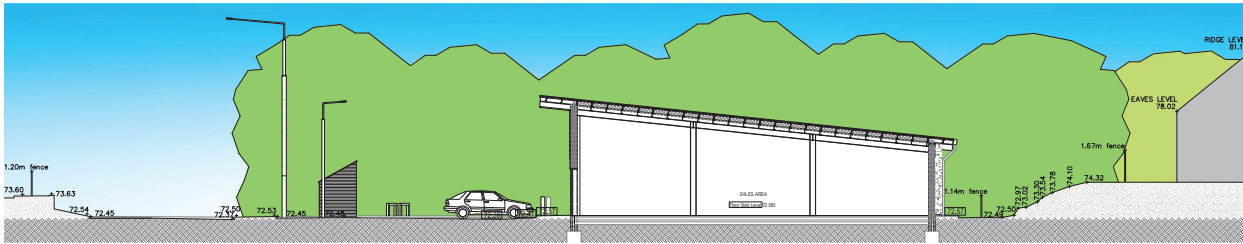
SECTION B-B 1:100
