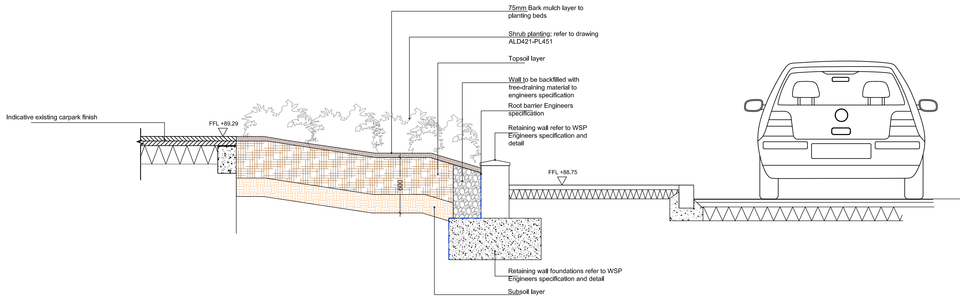
DETAIL 3: SECTION THROUGH LANDSCAPE AND RETAINING WALL 1:20 @ A1
