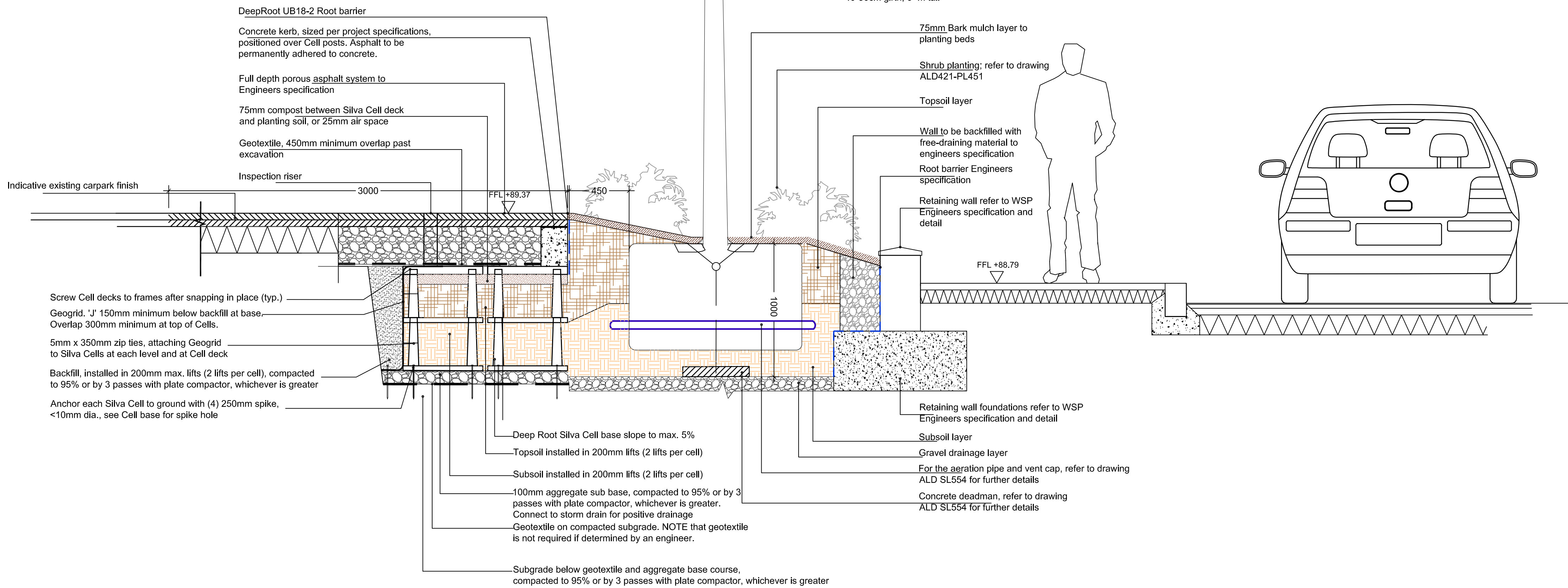
DETAIL 2: SECTION THROUGH SILVA CELL TREE PIT AND RETAINING WALL 1:20 @ A1
