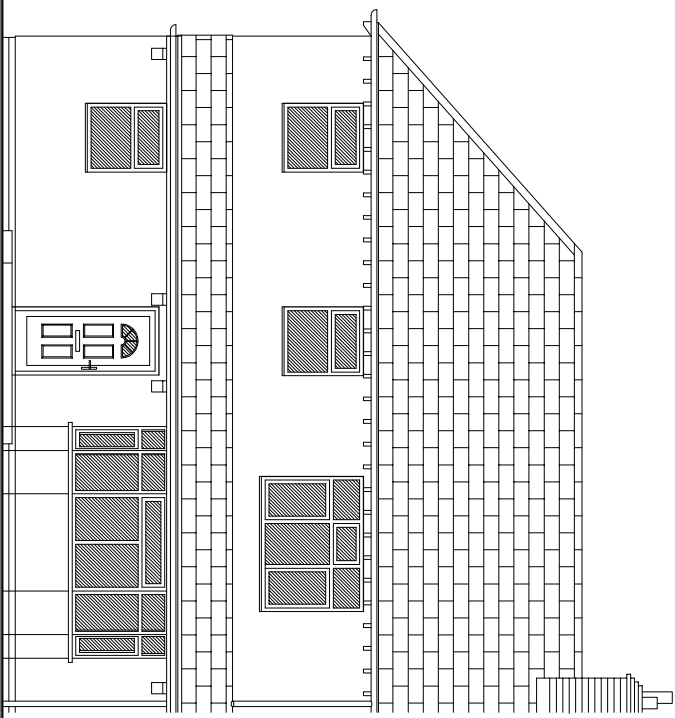
Proposed Kenyon Av. Elevation
