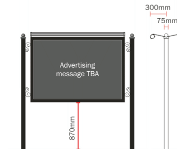
Sign 'F' Scale 1:50 Description - Double sided twin post sign Materials - Aluminium, corex and vinyl Illumination - Pelmet lights Panel size - 1,760mm x 1,210mm Note: Cap height for 'T' of TBA = 94mm
