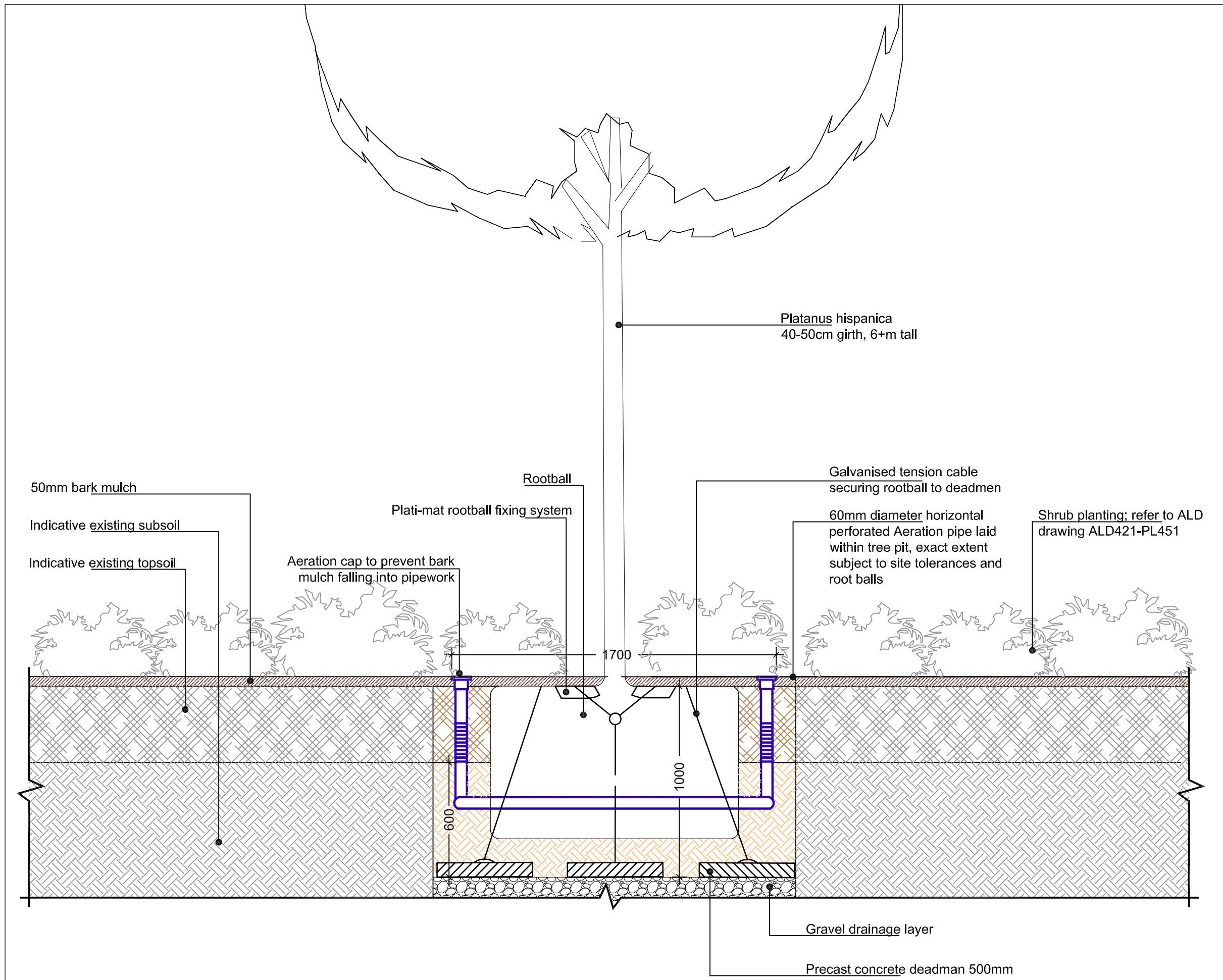
DETAIL 1: TYPICAL SECTION THROUGH TREE PIT AND ROOTBALL SHOWING AERATION / WATERING CAP. 1:20 @ A1
