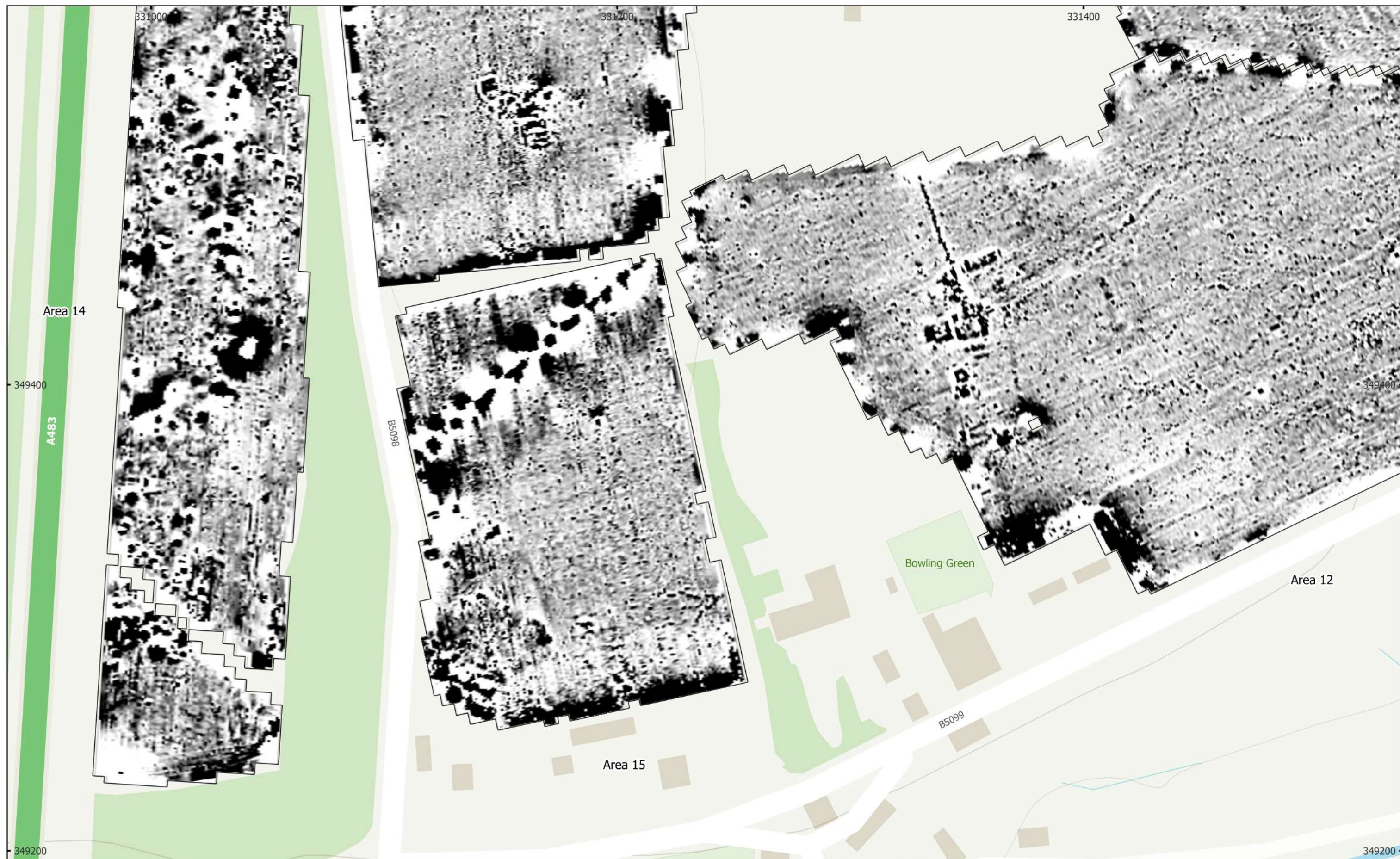
MSSJ1452: Land at Ruthin Road Figure 19 - Magnetic Gradient (South-western Areas) 1:1,500 @ A3 Copyright Magnitude Surveys Ltd 2022 Contains Ordnance Survey data © Crown Copyright and database right 2022
