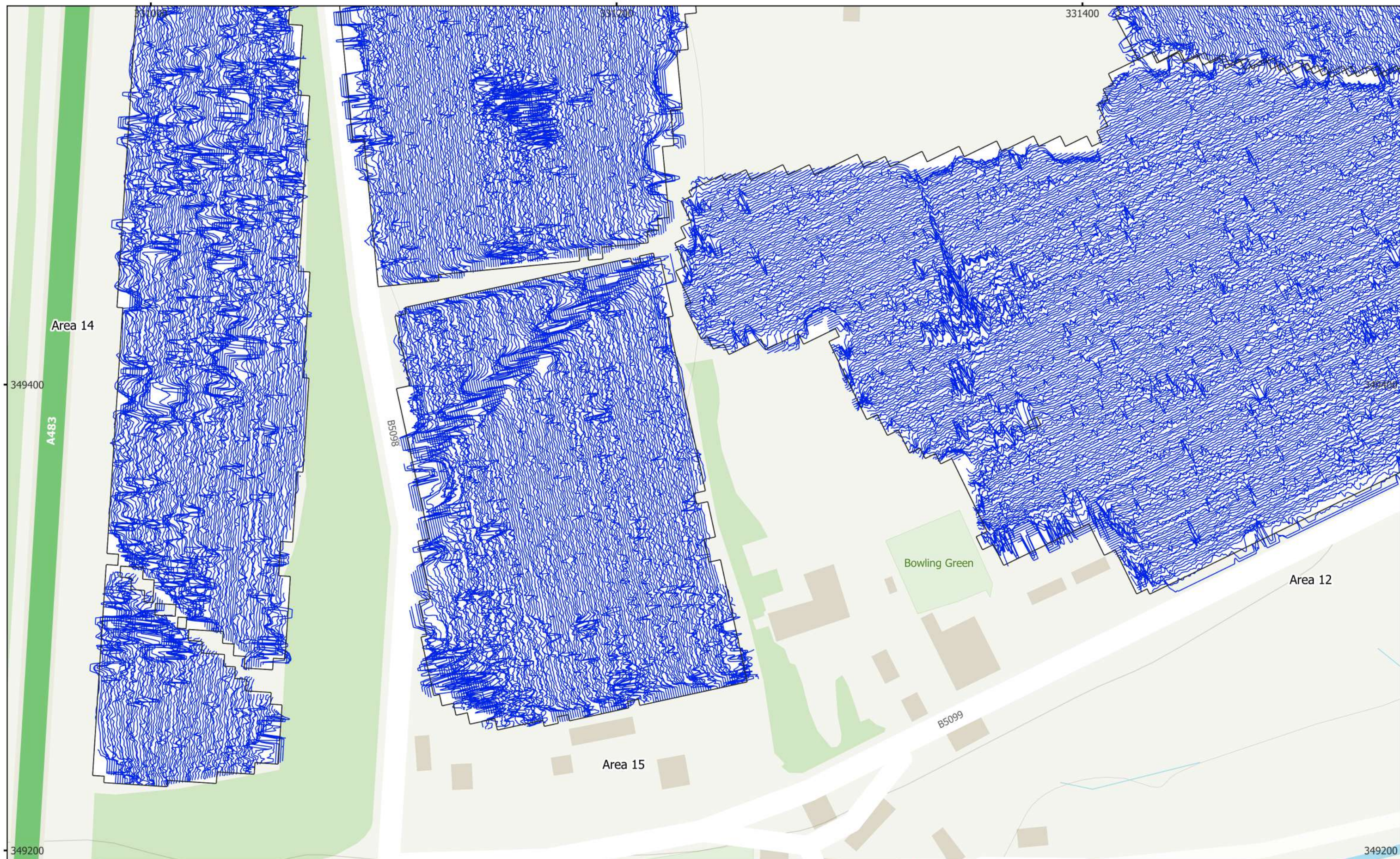
MSSJ1452: Land at Ruthin Road Figure 21 - XY Trace Plot (South-western Areas) 30nT/cm at 1:1,500 @ A3 Copyright Magnitude Surveys Ltd 2022 Contains Ordnance Survey data © Crown Copyright and database right 2022
