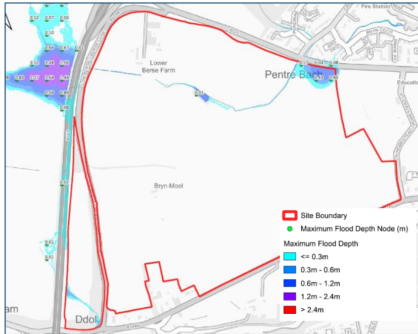
Figure 2 – Existing Scenario 1% AEP plus 45% CC Event – Flood Depths (m)
