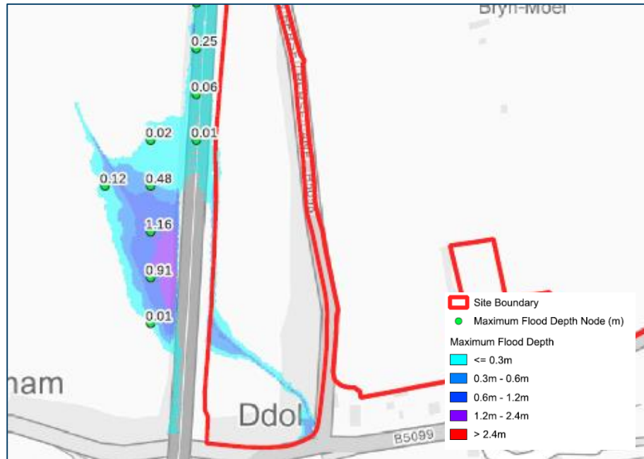
Figure 3 – Existing Scenario 0.1% AEP plus 45% CC Event - South-Western Watercourse – Flood Depths (m)
