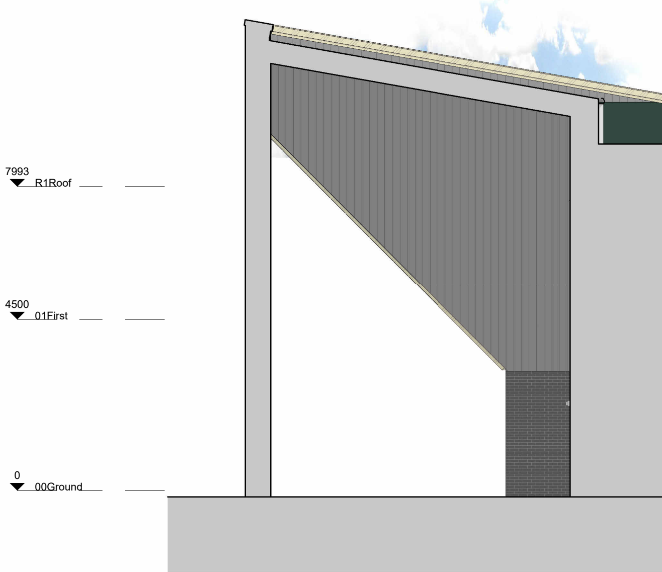
7 GA_Elevation_Proposed_07 Scale: 1 : 100
