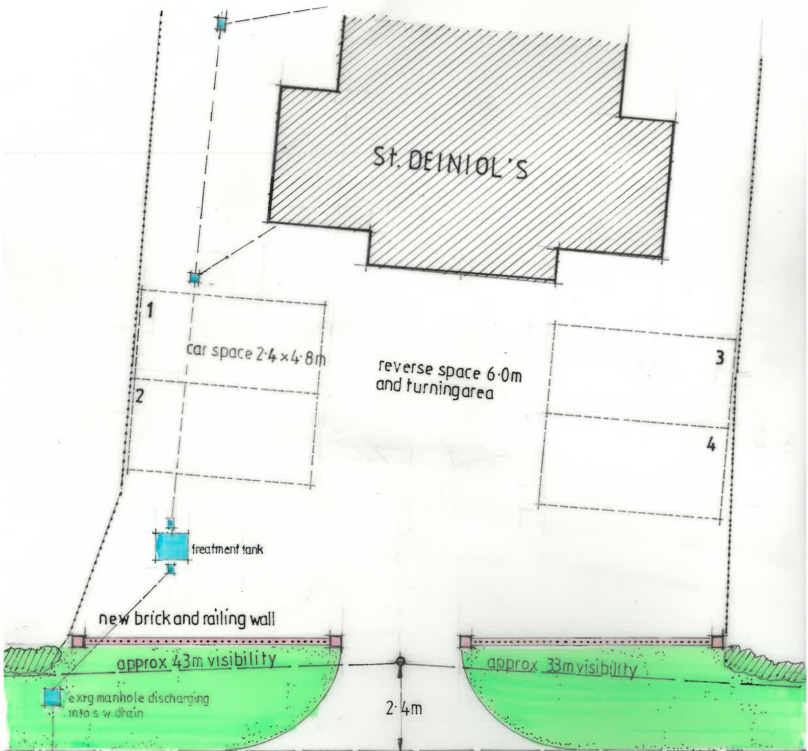
1. 100 block plan
