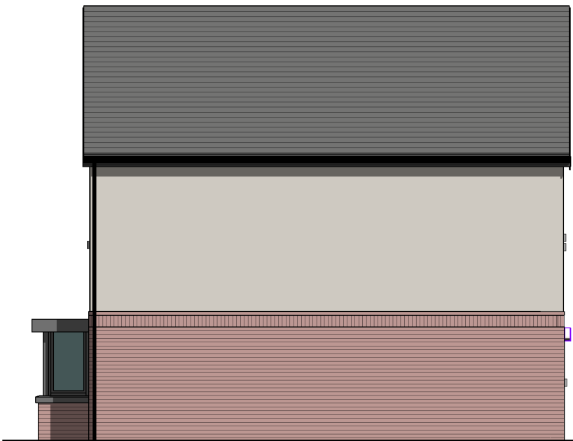
SIDE ELEVATION 1 : 100
