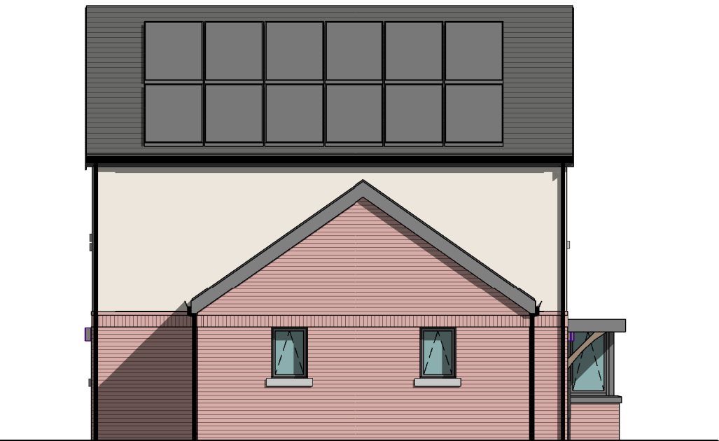
SIDE ELEVATIONa 1 : 100
