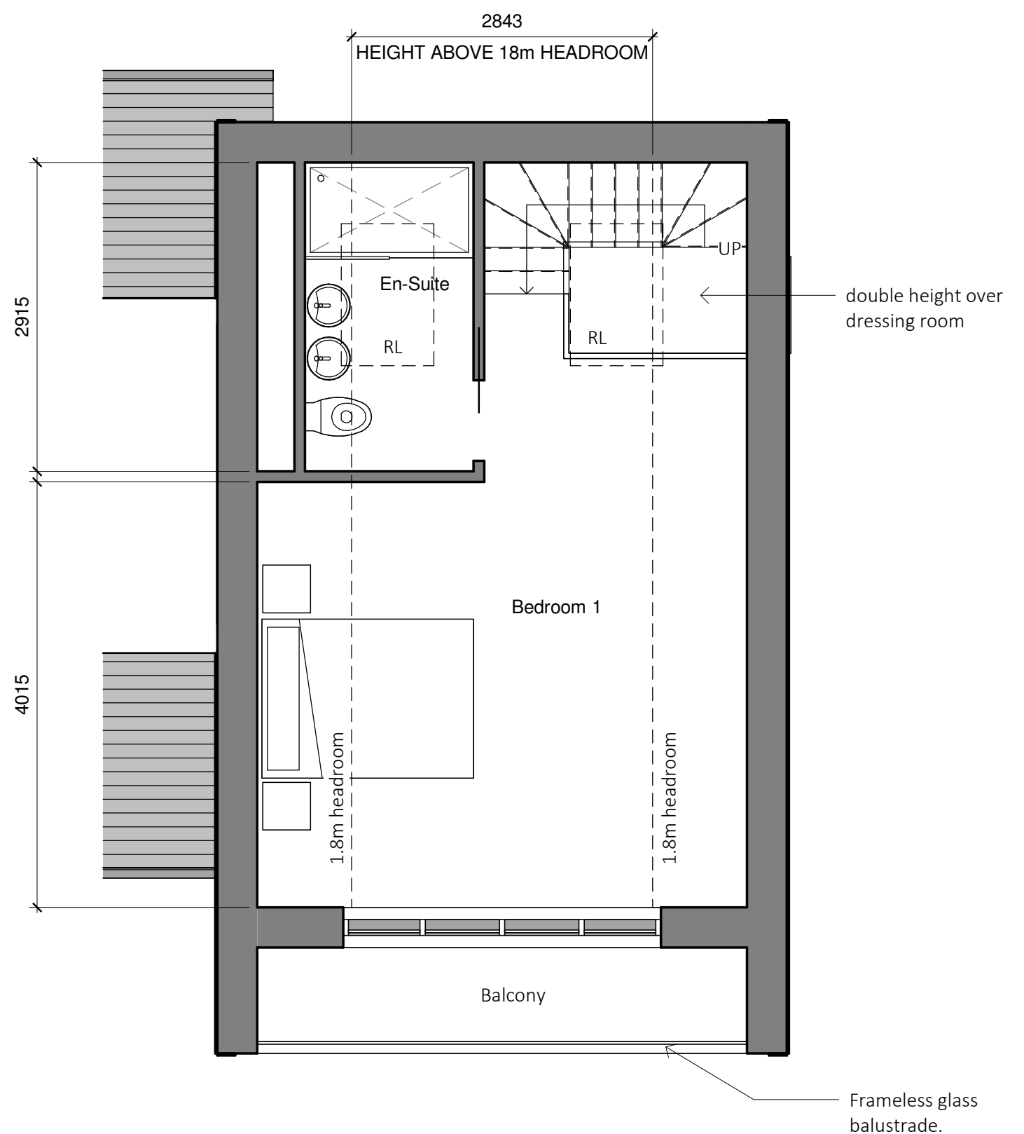
Proposed Loft Level 1 : 50
