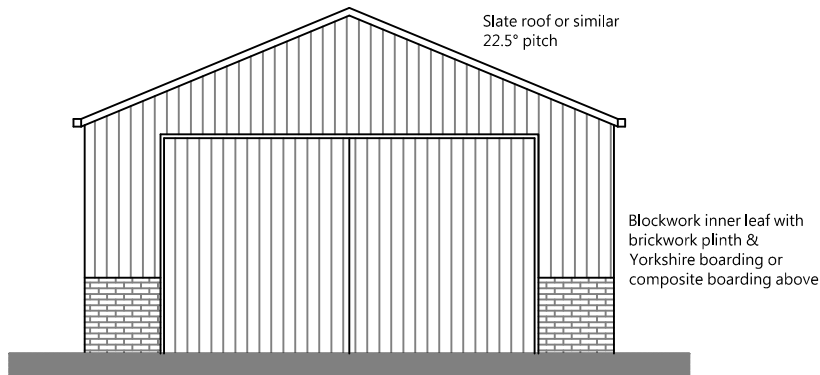
PROPOSED NORTH WEST ELEVATION
