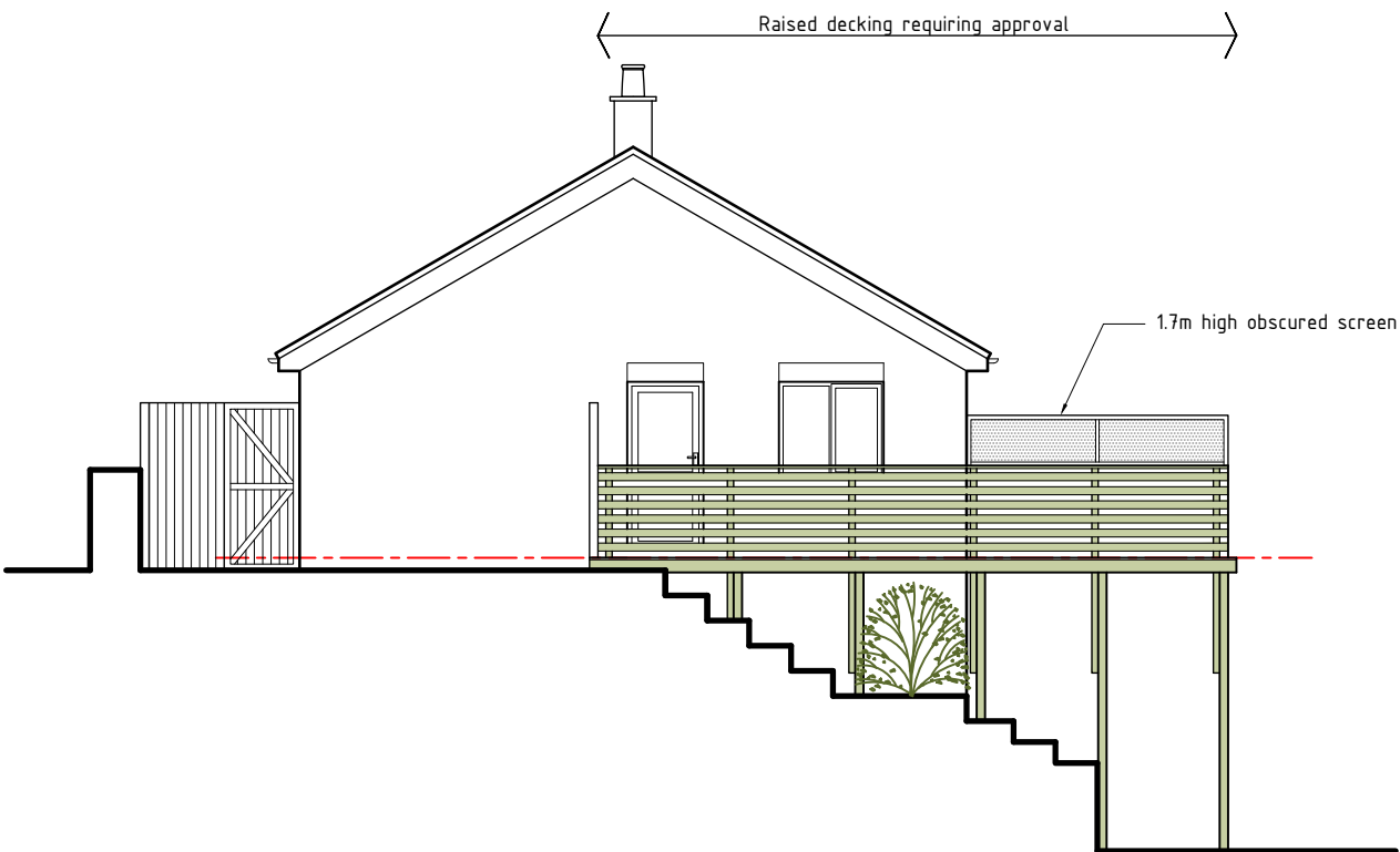
Side-01 elevation 1:100
