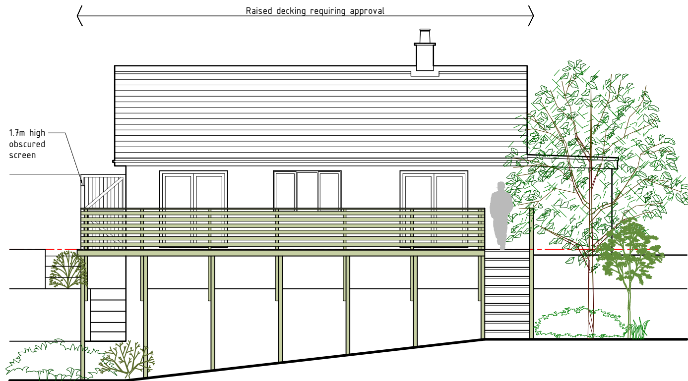
Front elevation 1:100
