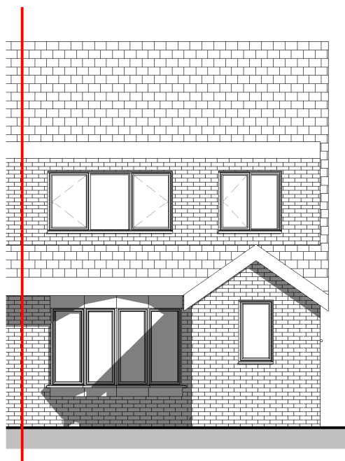
Front Elevation 1 : 100
