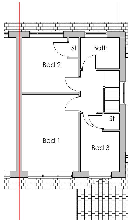
First Floor 1 : 100
