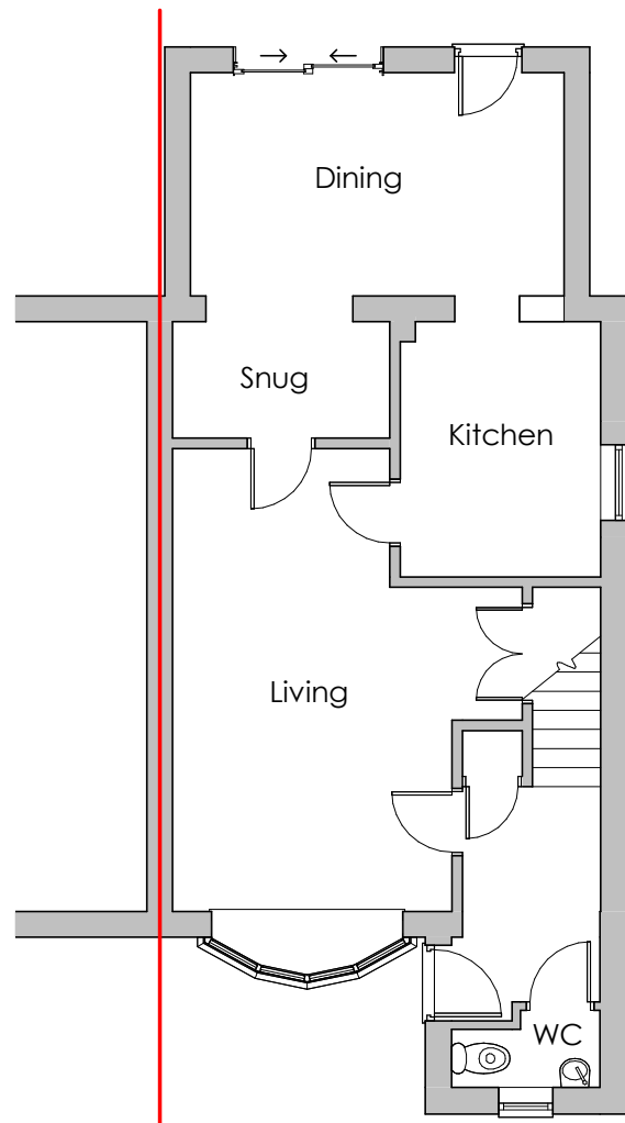
Ground Floor 1 : 100
