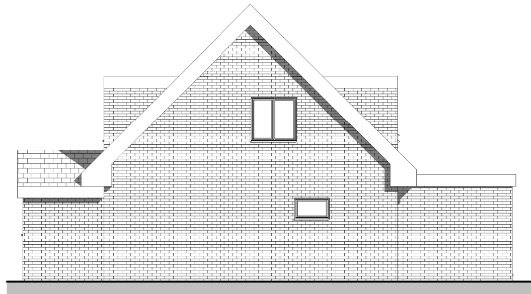
Side Elevation
