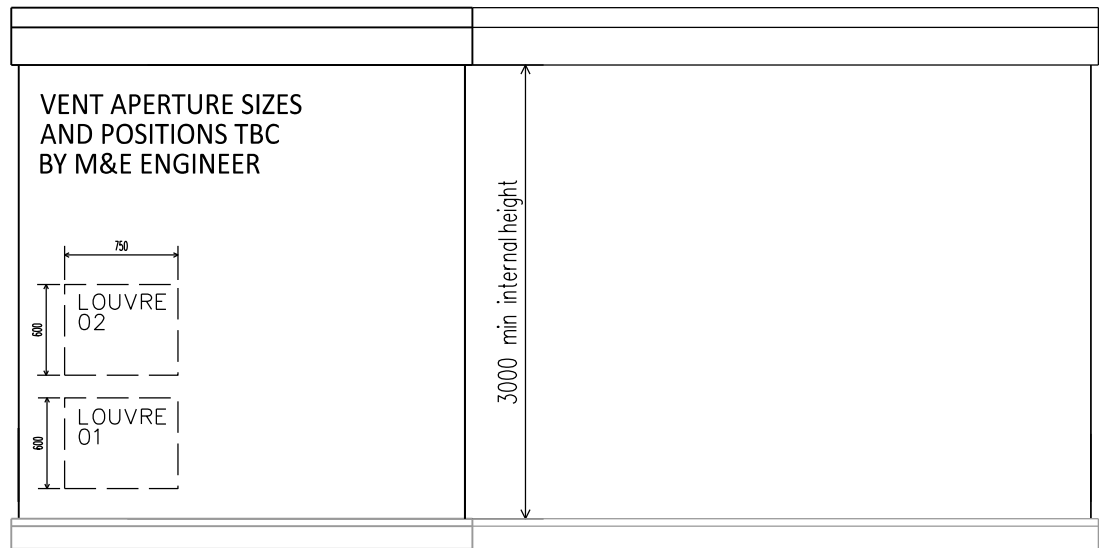
AHU Enclosure Elevation D
