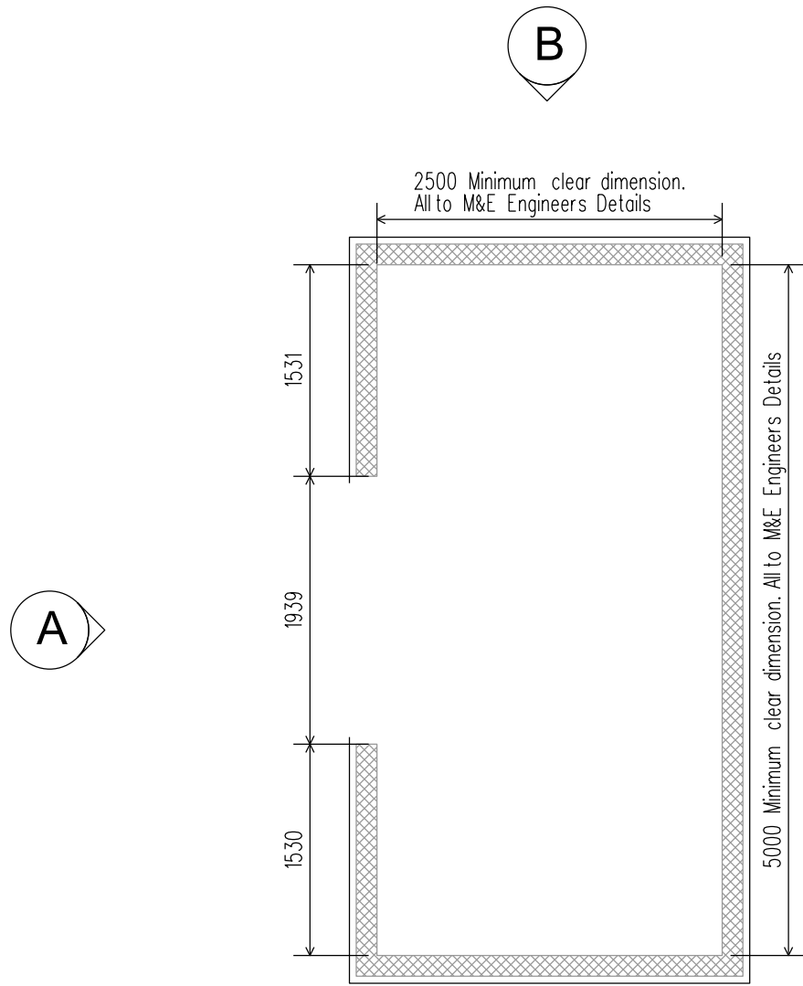
UPS Enclosure Plan
