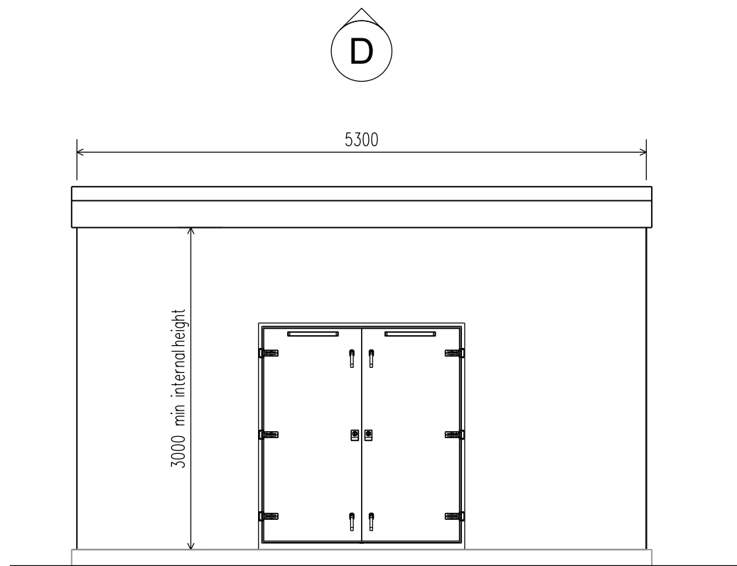
UPS Enclosure Elevation A
