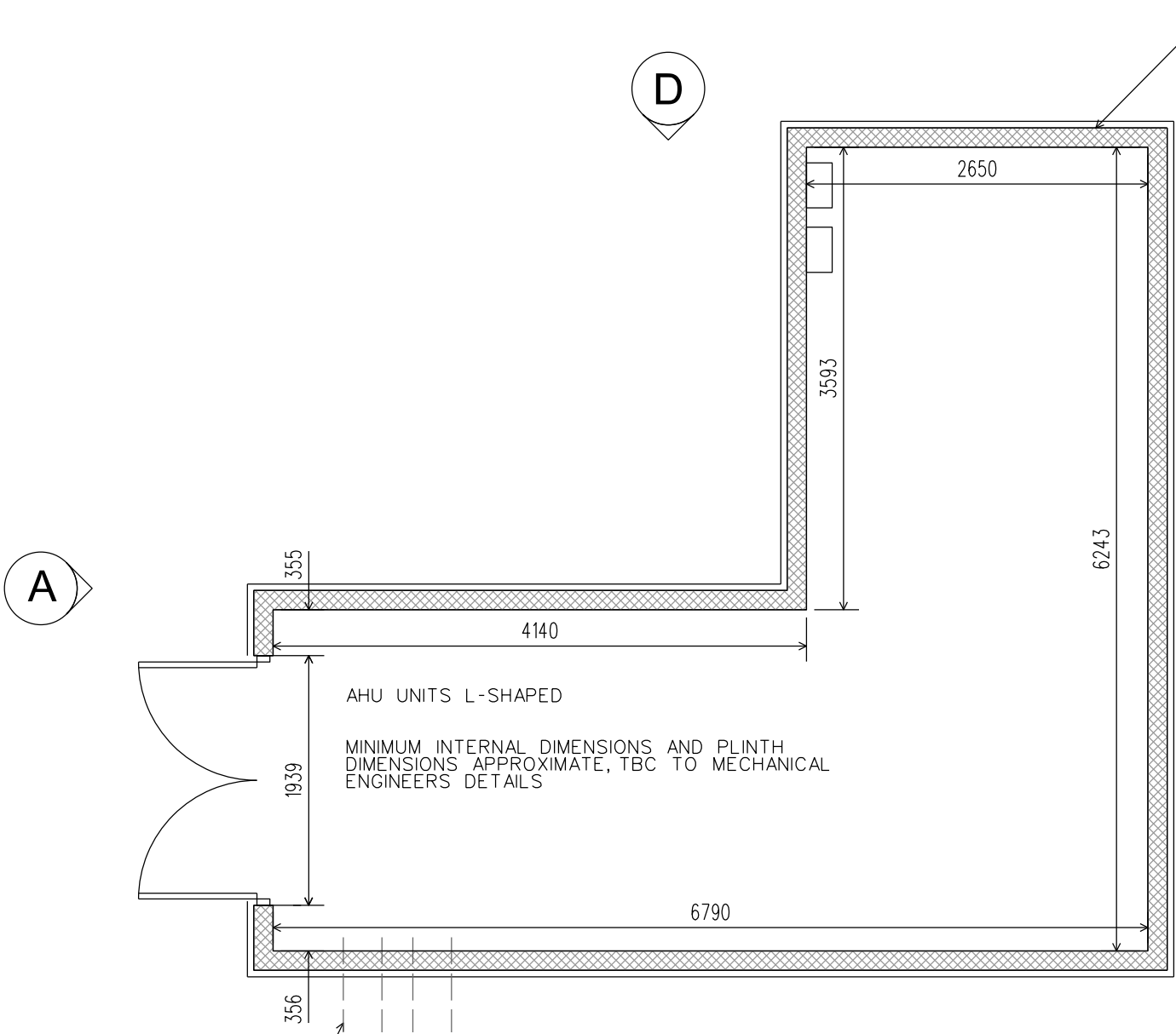
AHU Enclosure Plan
