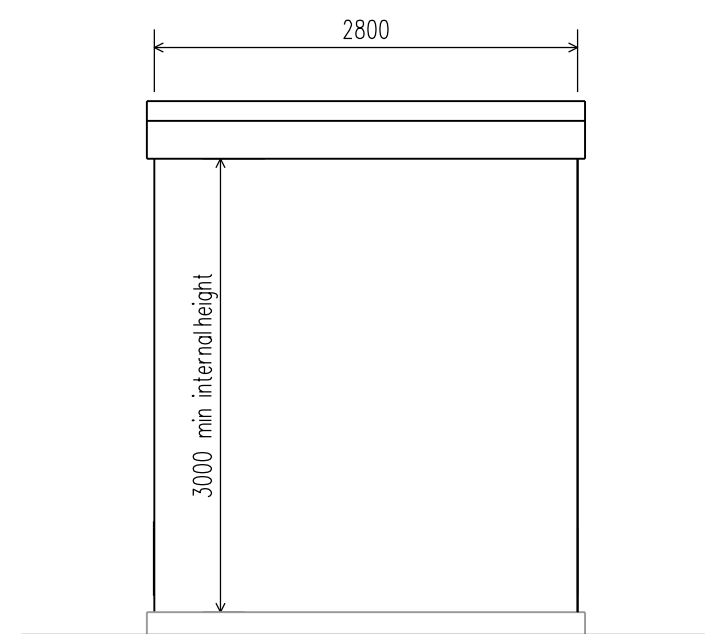
UPS Enclosure Elevation D
