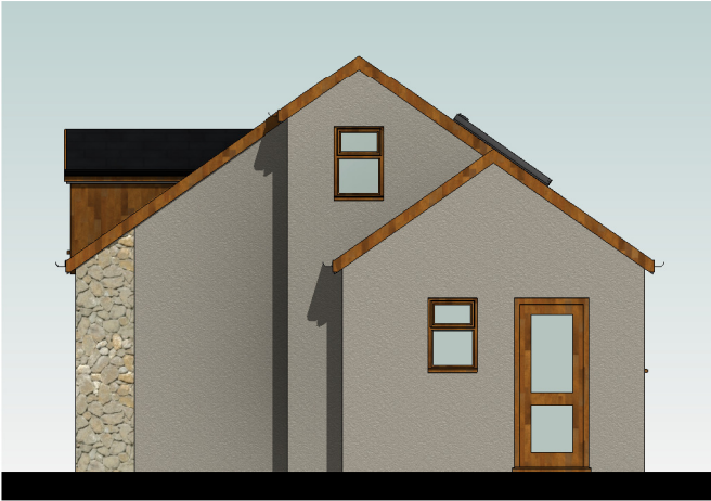
Proposed Side Elevation 1 : 100
