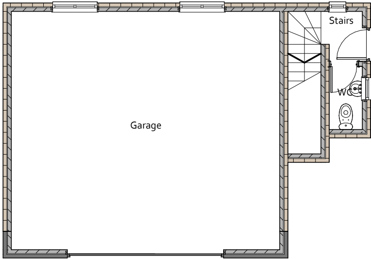
Proposed Ground Floor Plan 1 : 100
