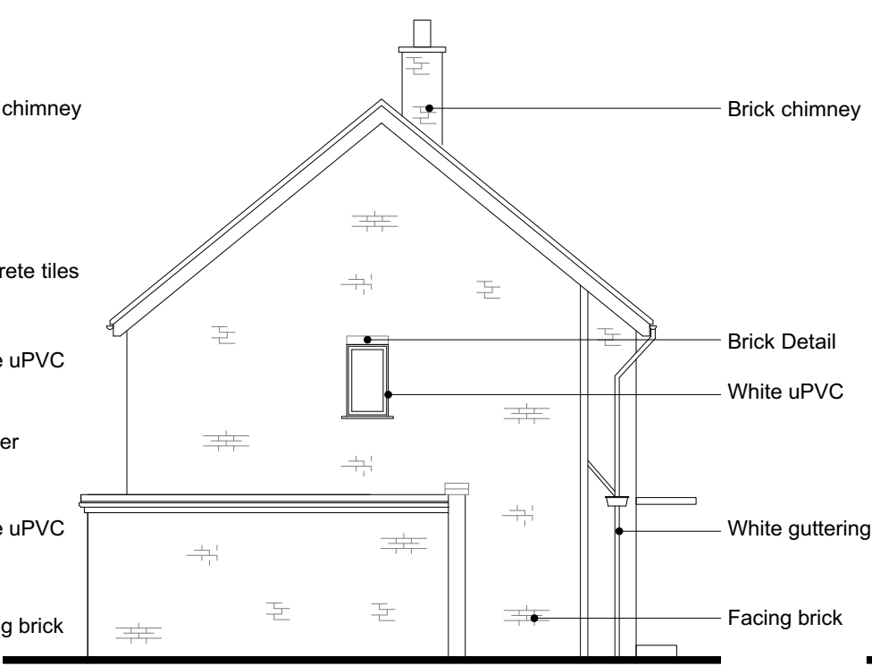
Existing Side Elevation View B - 1:100
