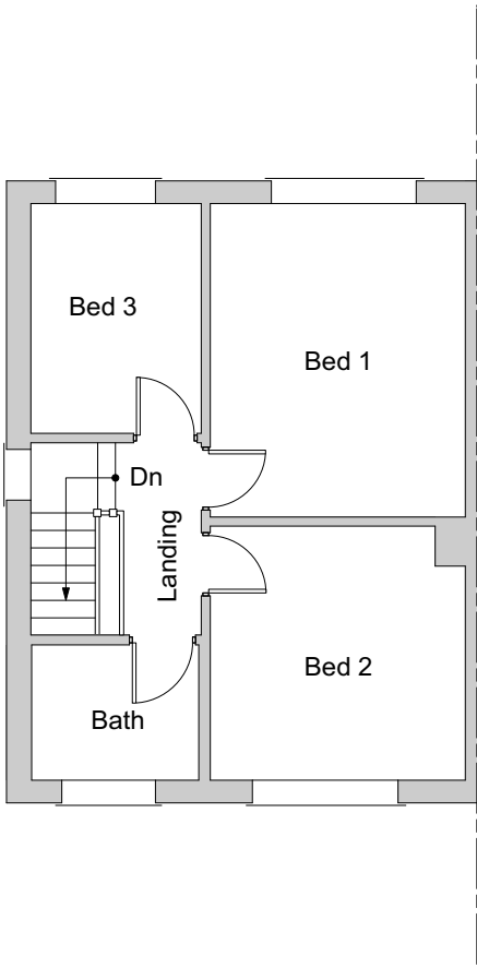
Existing First Floor Plan 1:100
