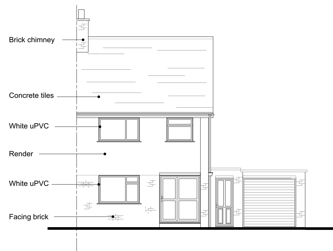
Existing Front Elevation View A - 1:100
