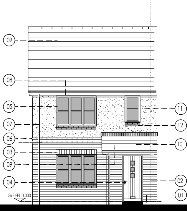
Front Elevation Brick & Render Elevational Treatment
