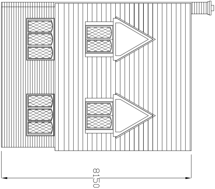
NORTH ELEVATION
