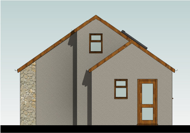
Existing Side Elevation 1 : 100
