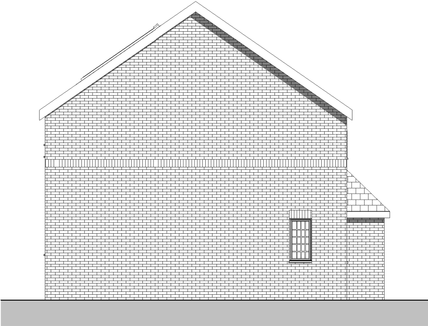
Side Elevation 1 : 100
