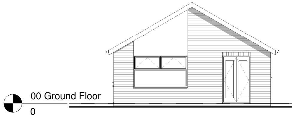
South Elevation 1 : 100
