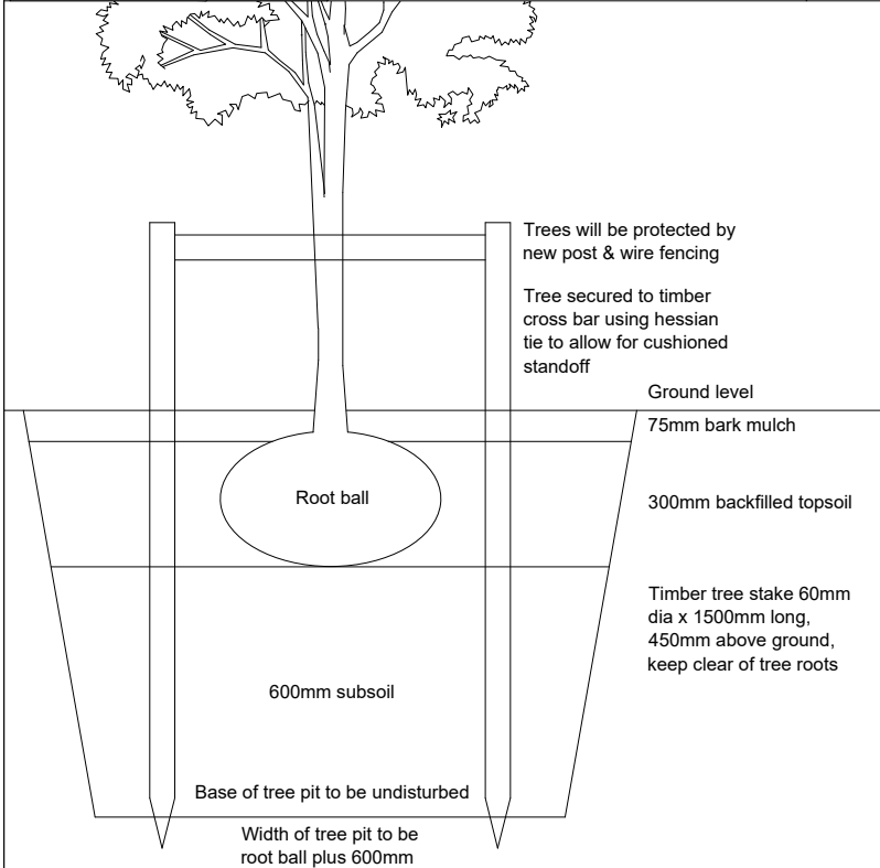
TREE PIT DETAIL 1:20
