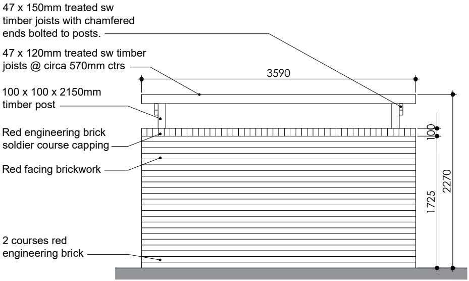
SIDE ELEVATION
