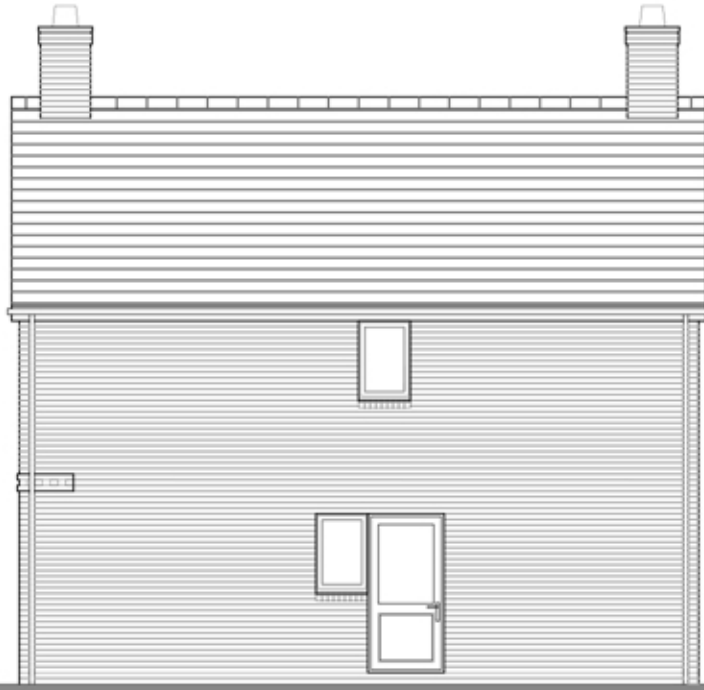
Rear Elevation
